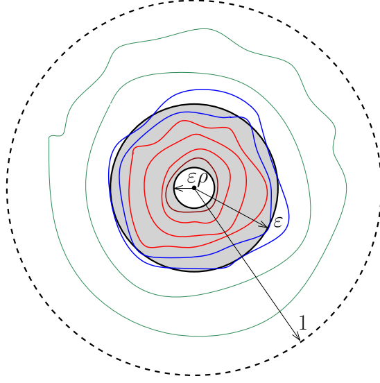
FIGURE 11. The whole set of loops in the unit disk \mathbb{D} is counted by \mathcal{N}_0(\epsilon\rho) , with \rho = \epsilon_1\epsilon_2 . The set of loops contained in the inner annulus, as counted by \widehat{\mathcal{N}}(\epsilon\rho) (resp. the set of intersecting loops, as counted by \mathcal{N}_\cap(\epsilon) ) appears in red (resp. blue).
