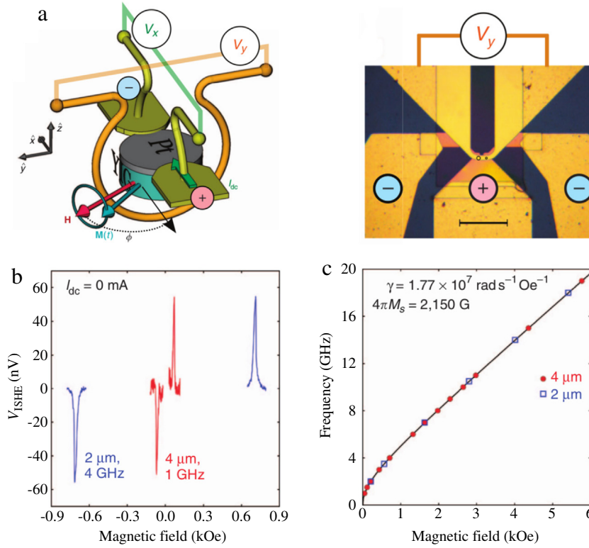
Fig. 9. ISHE-based FMR spectroscopy of YIG/Pt microdisks. (a) Sketch of the experiment with the micrograph of the device with two microdisks. Scale bar is 50 \mu\text{m} . The in-plane bias field H is oriented at an azimuthal angle \varphi = 90^\circ with respect to the direction of the dc current flowing in the Pt electrode. The excitation field h_{\text{rf}} is produced by the rf voltage V_y applied to the inductive loop. The dc voltage V_x across Pt is monitored as a function of the magnetic field strength. (b) ISHE-detected FMR spectra of the 4 \mu\text{m} and 2 \mu\text{m} YIG(20 nm)/Pt(8 nm) disks at 1 GHz and 4 GHz, respectively. (c) Magnetic-field dependence of frequency of the main FMR mode of the microdisks. The continuous line is a fit of the experimental data based on the Kittel law [36].
