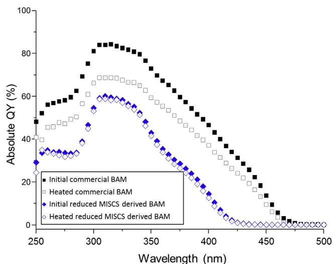
Fig. 14. Evolution of the room temperature absolute photoluminescence quantum yield versus excitation wavelength for combustion-derived and commercial BAM:Eu before ("initial") and after ("heated") 15 h at 170 °C under 365 nm.
