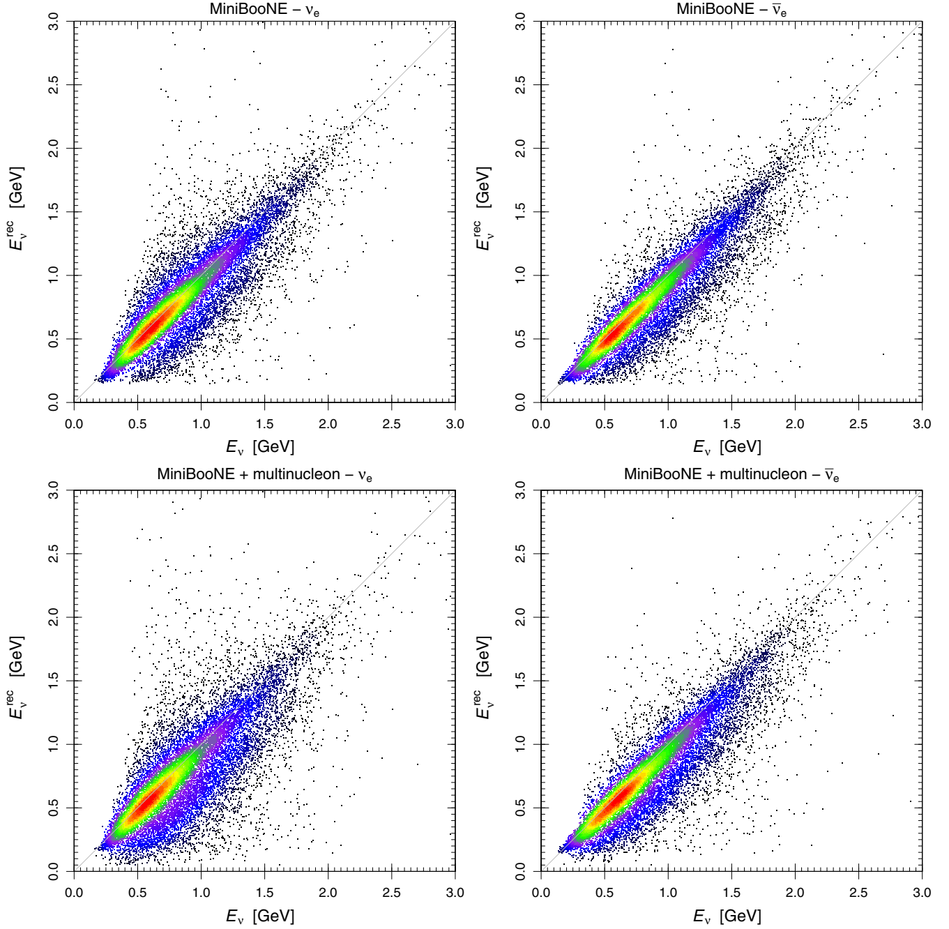
FIG. 1. Scatter plots which show the correlation between the true neutrino energy E_{\nu} and the reconstructed neutrino energy E_{\nu}^{\text{rec}} in the original [96] MiniBooNE muon-to-electron neutrino and antineutrino Monte Carlo full transmutation events (upper plots) and in the events modified with the contribution of multinucleon interactions (lower plots). The color sequence (black, blue, magenta, green, yellow, and red) indicates an increasing density of points.
