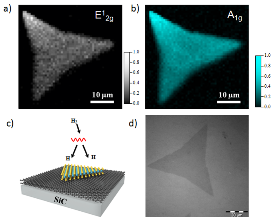
Figure 1. (a,b) Micro-Raman maps of E_{12g} and A_{1g} peaks of the \text{MoS}_2 on epitaxial graphene. (c) Schematic illustration of our current method for hydrogen-doped \text{MoS}_2 . (d) Typical optical image of a hydrogenated \text{MoS}_2 flake on epitaxial graphene/SiC.
