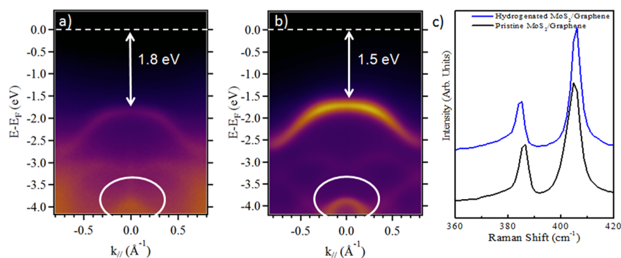
Figure 4. (a,b) ARPES measurements at room temperature of pristine MoS 2 /graphene at h\nu = 50 eV and hydrogenated MoS 2 /graphene heterostructure at h\nu = 100 eV, respectively along the graphene \Gamma K direction. The Fermi level position is located at the zero of the binding energy (marked as a white dashed line), the white circles highlight the shift in the position of the band located at around -4 eV. (c) Comparison between the Raman spectra of MoS 2 before (in black line) and after (in blue line) hydrogenation.
