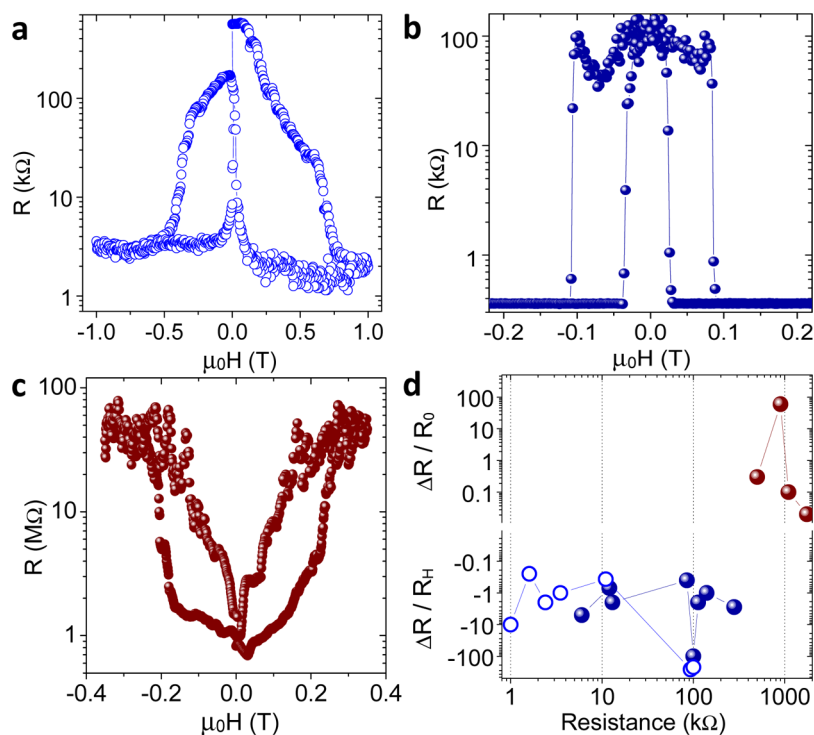
Figure 3. (a–c) Large MR measured in gas-stabilized Pt nanowires with initial resistance R \geq 100 k \Omega measured at 4 K (a,c) and 77 K (b). Data in (c) averaged over 10 mT. (d) Variation of the MR as a function of the nanowire resistance measured at 4 K (open symbols) and 77 K (filled symbols). The MR turns from negative (reduced resistance in a magnetic field—blue) to positive (increased resistance—red) for structures with resistance above \sim 300 k \Omega .
