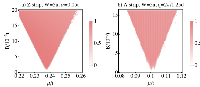
Figure 14: Dependence of the MP with B and \mu for a strip with W = 5a , L = 1557a , \Delta = 0.001t for a) a Z strip with \alpha = 0.05t . Note the formation of Majoranas for a region centered around \mu = 0.23 - 0.24t , for B > 0.001t b) an A strip with q = 5 \approx 2\pi/(1.25d) . Note the formation of Majoranas for a region centered around \mu = 0.1t , for B > 0.001t .
