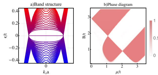
Figure 9: a) Band structure for a graphene nanoribbon with a magnetic field rotating in the plane of the ribbon, with an wave vector 2\pi/5d parallel to the edges of the ribbon, for \mu = 3t , B = t and \Delta = 0.2t , W = 86a . b) Phase diagram as a function of \mu and B for \Delta = 0.2t , W = 173a .
