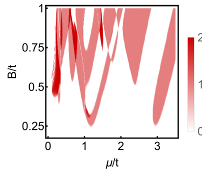
Figure 8: The total MP as a function of the chemical potential and a magnetic field perpendicular to the plane for Z strips. We consider a ribbon of width of W = 5a , for \alpha = 0.5t and \Delta = 0.2t , same as in Fig. 3b) for an in-plane field.
