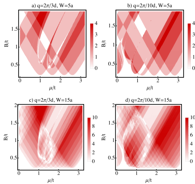
Figure 10: A strips: Topological phase diagrams for W = 5a (top) and W = 15a (bottom). We consider a wavevector of q = 2\pi/3d (left column, L = 86a ), and q = 2\pi/10d (right column, b) L = 346a and d) L = 173a ). We take \Delta = 0.2t .
