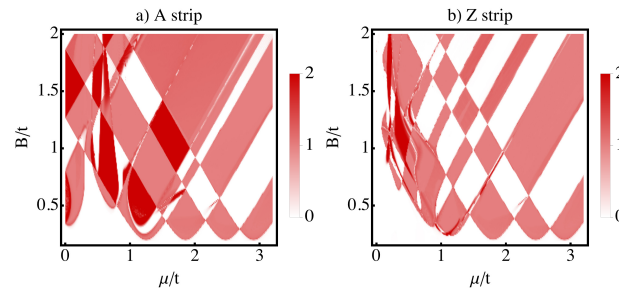
Figure 3: The total MP as a function of the chemical potential and magnetic field for A strips (left panel) and Z strips (right panel). We consider a ribbon of width of W = 5a and length L = 520a , for \alpha = 0.5t and \Delta = 0.2t .
