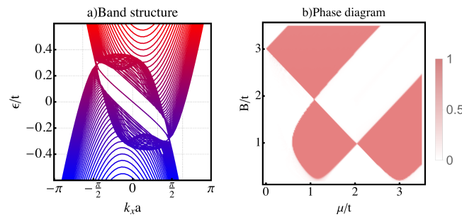
Figure 2: a) The band structure for a zigzag ribbon of W = 86a , with in-plane field for \mu = 2.9t , B_y = 0.5t , \alpha = 0.5t , \Delta = 0.2t . Note the formation of chiral Majorana states and the overall gapless character of the band structure. b) Topological phase diagram for a zigzag ribbon of W = 260a as a function of \mu and B for \alpha = 0.5t , and \Delta = 0.5t . We plot the MP of the lowest energy state, thus a value of 1 corresponds to a topological phase (pink), while a value of 0 to the trivial one (white).
