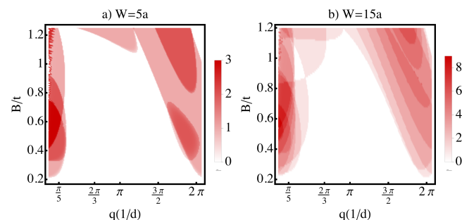
Figure 13: a) Dependence of total MP with the amplitude of the magnetic field B (in units of t ) and q (in units of 2\pi/d ) for Z strips. Use a) W = 5a and b) W = 15a strips, with L = 173a , and \Delta = 0.2t
