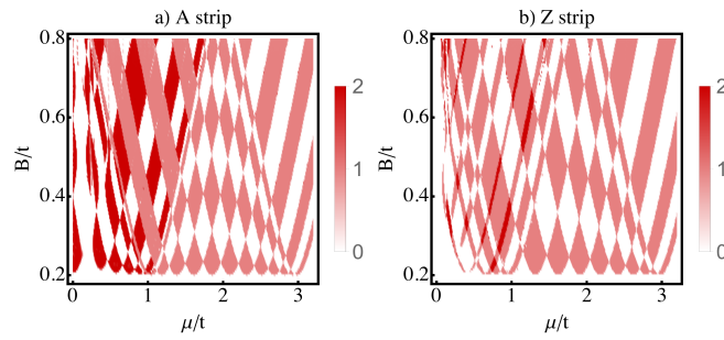
Figure 6: The total MP as a function of the chemical potential and magnetic field for A strips (left panel) and Z strips (right panel). We take W = 15a , L = 432a , \alpha = 0.1t and \Delta = 0.2t
