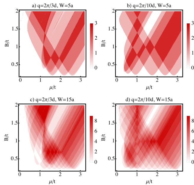
Figure 12: Z strips: Topological phase diagrams for strips with W = 5a (upper row) and W = 15a (lower row). We consider a wavevector of q = 2\pi/3d (left column, L = 86a ), and q = 2\pi/10d (right column, b) L = 346a and d) L = 173a ). As before we take \Delta = 0.2t .
