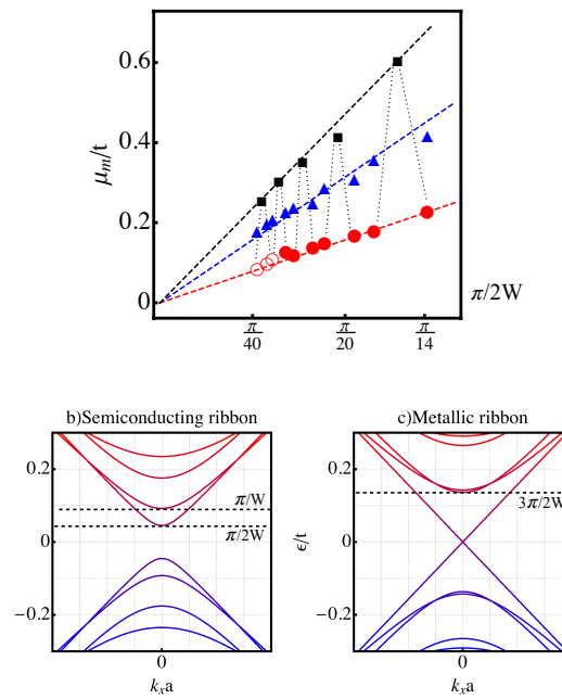
Figure 7: a) The dependence of the chemical potential required to form MBS as a function of ribbon width. The red circles correspond to semiconducting ribbons, while the black squares to metallic ones. The blue triangles correspond to the second lowest value of the required chemical potential. For all these points we consider the formation of MBS at V_Z \approx \Delta . The empty red circles correspond to the formation of MBS at V_Z \approx \Delta . The dashed red line corresponds to the gap of a semiconducting ribbon E_{\text{gap-semiconductor}} = \pi/2W , the dashed black line to the minimum of the second band of a metallic ribbon E_{\text{second-band-metal}} = 3\pi/2W , while the blue dashed line to the minimum of the second band for a semiconducting ribbon E_{\text{second-band-semiconductor}} = \pi/W . b) The band structure for a parent infinite semiconducting strip of width W . c) The band structure for a parent infinite metallic strip of width W .
