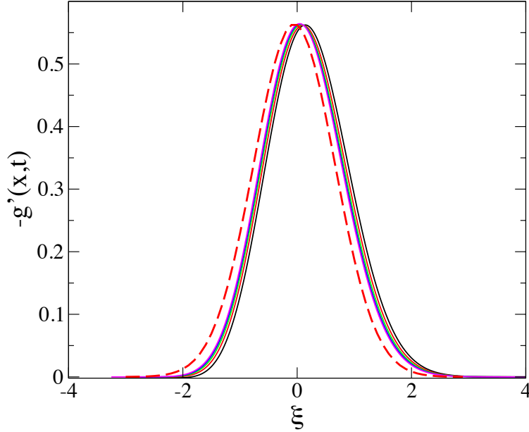
Figure 8. Same data as in figure 3 against \xi , compared to the Gaussian e^{-\xi^2}/\sqrt{\pi} (dashes). This function is normalised to unity with respect to \xi .
