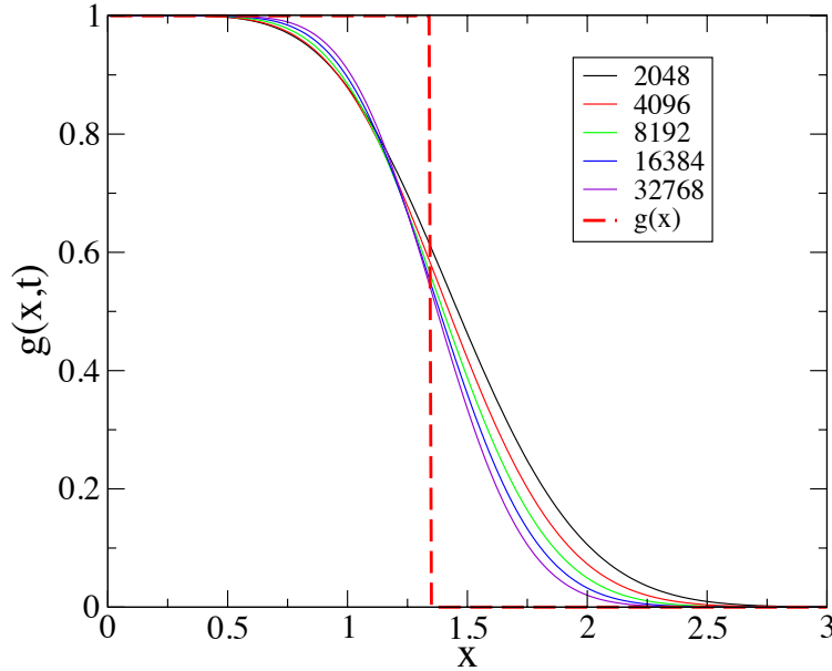
Figure 4. Function g(x, t) against x for t = 2048, 4096, \dots, 32768 , obtained from the data of figure 2. The discontinuous curve is the limiting scaling function g(x) . The discontinuity is at x_0 = (b(1 + \sigma))^{1/(1+\sigma)} , i.e., x_0 = 1.341 \dots with \sigma = 0.6, b = 1 .
