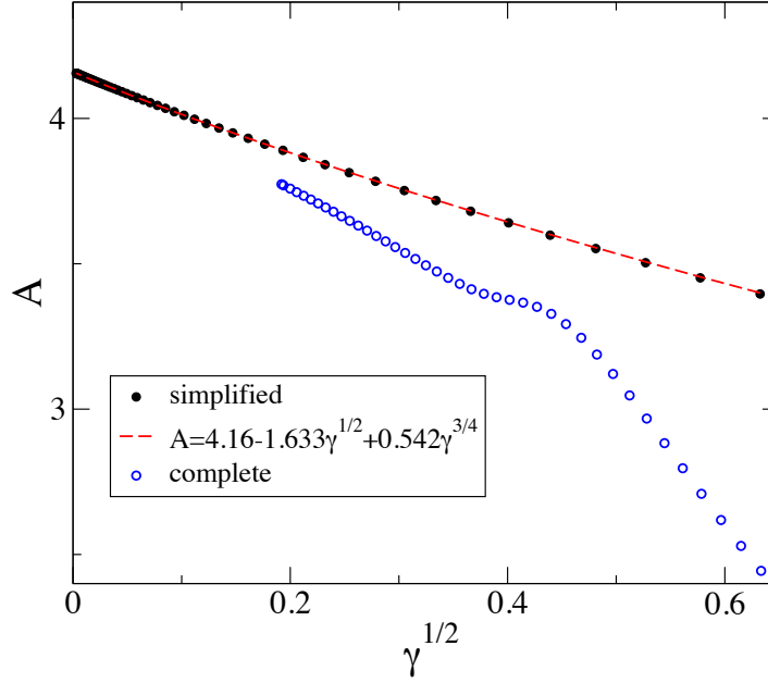
Figure 12. Upper curve: comparison between the amplitude A corresponding to the solutions, depicted in figure 11, of the simplified equation (6.10) (black dots) and the prediction (6.27) (red dashes). Lower curve: amplitude A obtained by numerical integration of the master equation (3.1) (the continuum limit of which is the complete equation (5.19)) (open blue dots).
