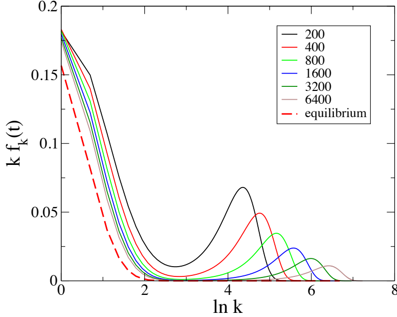
Figure 9. Product k f_k(t) against \ln k for t = 200, 400, \dots, 6400 . The dashed curve is the equilibrium distribution f_{k,\text{eq}} . This figure substantiates the separation between the two time-occupancy regimes (I) and (II). Here \sigma = 1/2, b = 4, \rho_c \approx 0.306, \rho = 20\rho_c .
