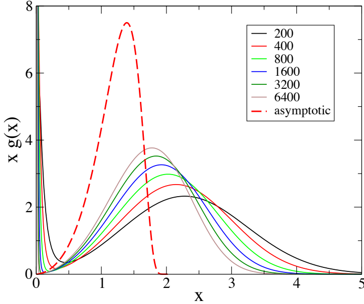
Figure 10. Same as figure 9 against the scaling variable x . The asymptotic dashed curve xg(x) (6.4) is normalised according to (5.12).
