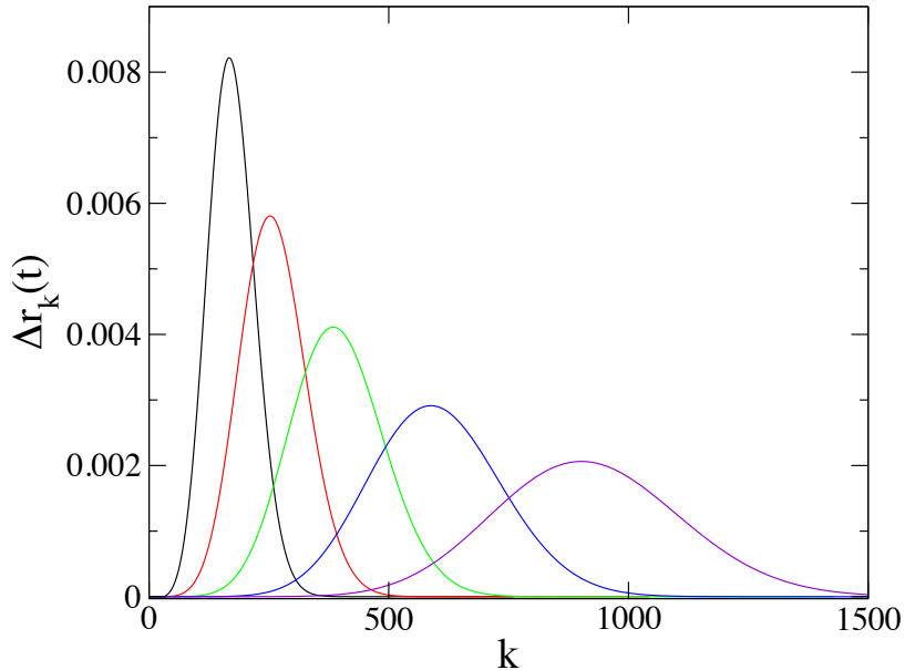
Figure 3. Differences r_k(t) - r_{k+1}(t) for t = 2048, 4096, \dots, 32768 , obtained from the data of figure 2.
