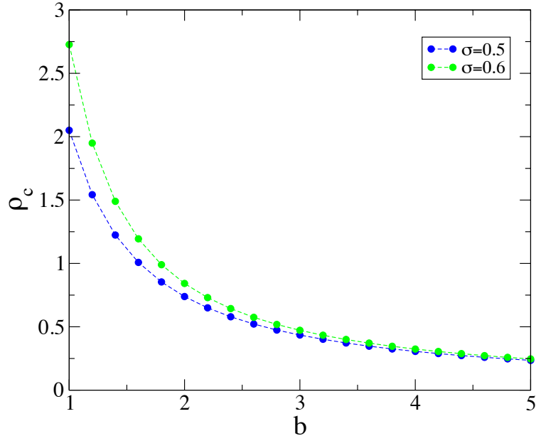
Figure 1. Critical density \rho_c for the ZRP (2.3) for two values of \sigma .
