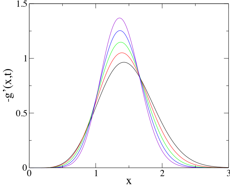
Figure 5. Function -g'(x, t) for t = 2048, 4096, \dots, 32768 , obtained from the data of figure 4.
