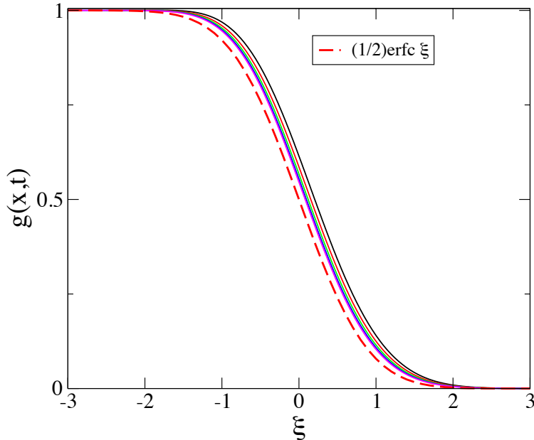
Figure 7. Same data as in figure 2, against scaling variable \xi defined in (4.30), compared to the bulk scaling function (1/2)\text{erfc } \xi (dashes).
