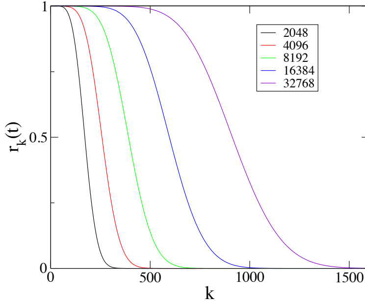
Figure 2. Critical ratio r_k(t) = f_k(t)/f_{k,\text{eq}} for t = 2048, 4096, \dots, 32768 , obtained by numerical integration of the discrete master equation (3.1). Here \sigma = 0.6 , b = 1 .
