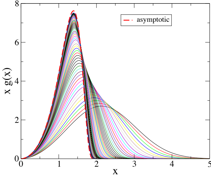
Figure 11. Solutions of the differential equation (6.10) obtained by numerical integration, for decreasing values of \gamma ( \sigma = 1/2, b = 4 ), ranging from \gamma = 0.4 ( t \approx 15 ) to \gamma \approx 8.5 \cdot 10^{-6} ( t \approx 1.62 \cdot 10^{15} ).
