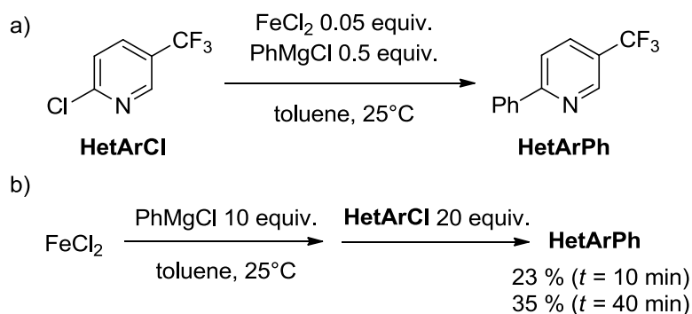
Scheme 10. Aryl-heteroaryl Kumada cross-coupling between PhMgCl and HetArCl investigated at room temperature (non-optimized conditions); a) catalytic one-pot conditions; b) step-by-step conditions with generation of \text{Fe}^0 prior to the addition of HetArCl . HetArPh yield calculated with respect to HetArCl .
