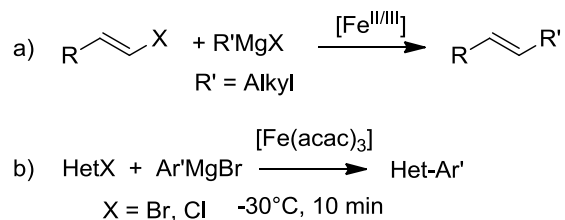
Scheme 1. Representative milestones in Fe-catalyzed C–C cross-couplings.
