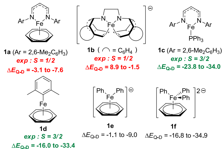
Scheme 8. \Delta E_{\text{Q-D}} = E_{\text{Q}} - E_{\text{D}} DFT quartet-doublet split (kcal.mol -1 , gas-phase, see SI for the assignments) for 1a , 1b , 1c , 1d , 1e and 1f ; basis sets for C, H, N, P : see SI.
