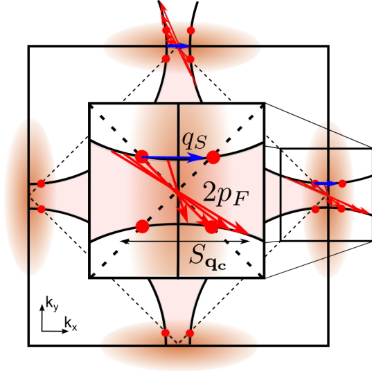
FIG. 1. (Color online) Fermi surface (solid line) in first BZ of the square lattice. The magnetic BZ is presented in dashed line and its intersection with the Fermi surface represents the position of the hot-spots (the red circle). The red solid arrow represents the 2\mathbf{p}_F vectors for two different points on the Fermi surface. The blue arrow represents the small ordering vector perpendicular to the zone edge \mathbf{q}_S , which is itself a 2\mathbf{p}_F -vector of the adjacent AN zone. The RES order parameter develops in the AN zone of the first BZ (orange area). S_{\mathbf{q}_c} is the size of the spread of the modulation vectors \mathbf{q}_c .
