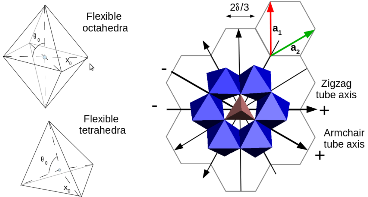
Figure 1. The model is based on flexible octahedra and tetrahedra having potential energy for center-vertex stretching E_s = \frac{1}{2} K_s (x - x_0)^2 and vertex-center-vertex bending E_b = \frac{1}{2} K_b (\theta - \theta_0)^2 . The values K_s , x_0 , K_b , and \theta_0 are not the same for octahedra and tetrahedra (see text). The octahedra are linked by edges in a Gibbsite-like 2D hexagonal structure. The tetrahedra are linked to 6 neighbors octahedra through three bonds. The positions in the 2D Gibbsite like structure are conveniently obtained with the two unit vectors \mathbf{a}_1 and \mathbf{a}_2 .
