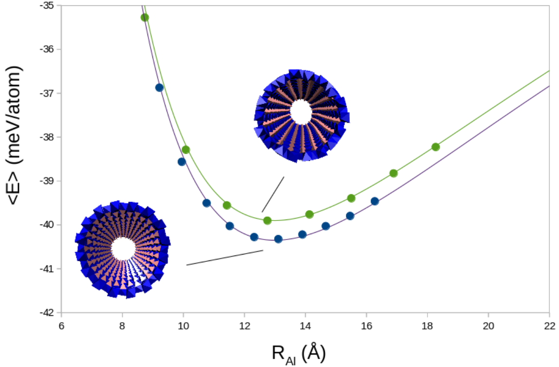
Figure3. Average potential energy of Zig-Zag and Armchair nanotubes with radius between 8 and 20 \text{\AA} . The energy is given in meV/atom where the atom number corresponds to vertices (counted only once when shared) and centers of tetrahedral and octahedral. The lines are fits of the curves \langle E \rangle = f(R) with the equation \langle E \rangle = E_0 + 0.5K_c(1/R - 1/R_0)^2 .
