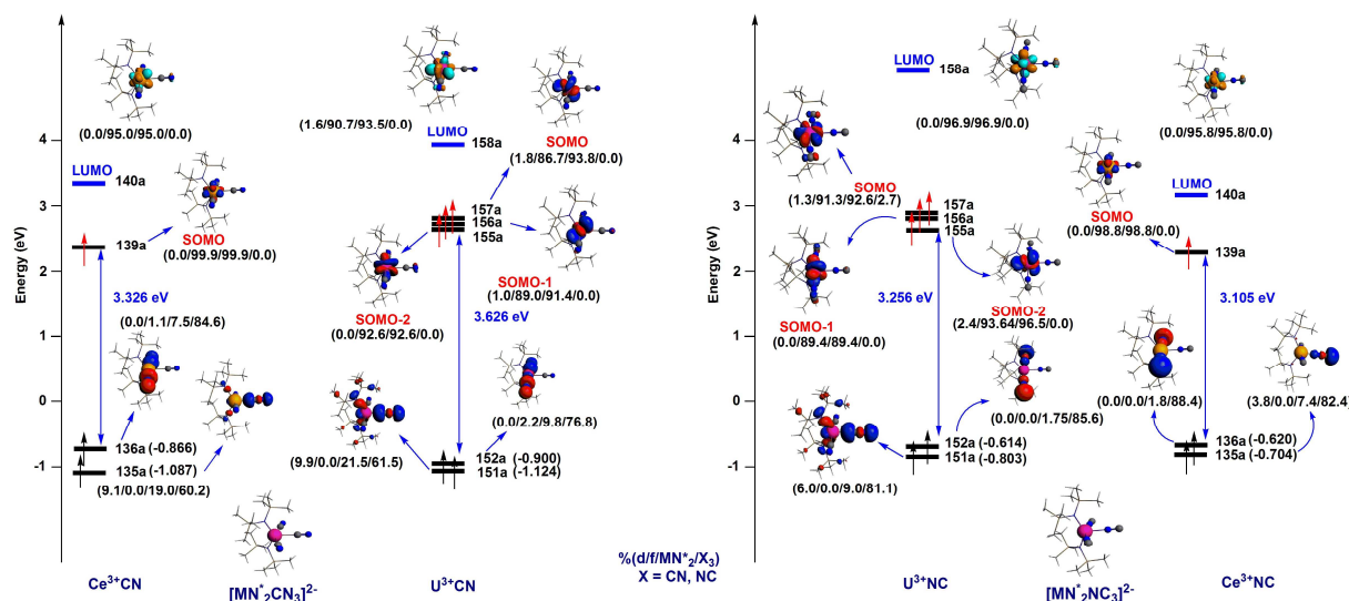
Fig. 4. ZORA/BP86/DZP \alpha spin-MO diagram for M–CN (left) and M–NC (right) [\text{MN}^*_2\text{X}_3]^{2-} ( \text{X} = \text{CN}/\text{NC} ) complexes ( C_1 symmetry). From the left to the right, the M d , M f , \text{ML}_2 , and \text{X}_3 percentage contributions are given in brackets. Contour values are \pm 0.03 ( \text{e}/\text{bohr}^3 ) ^{1/2} .
