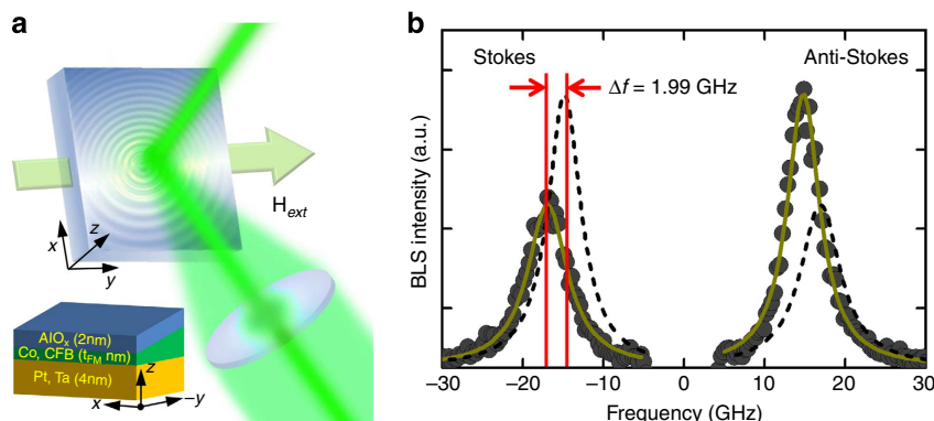
Figure 1 | The BLS measurements. (a) Schematic configuration of the BLS measurement. The external magnetic field is applied along the y-direction and a p-polarized laser beam excites two interfaces SWs along the x-direction. Inset: schematic picture of wedge-type sample geometry. (b) The BLS spectrum with a magnetic field H_{\text{ext}} = 0.69 T. The incident angle is fixed at \theta = 45^\circ ( k_x = 0.0167 \text{ nm}^{-1} ). To identify the frequency differences ( \Delta f ) between Stokes (negative frequency region) and anti-Stokes (positive frequency region), mirrored curves are drawn as black dashed line. The red vertical lines indicate the centre of the SW frequency and red arrows indicate the \Delta f , here 1.99 GHz. The black circles refer to the experimental result and dark yellow solid line is the Lorentzian fitting curve. The data accumulation time for each spectrum is about 60 min.
