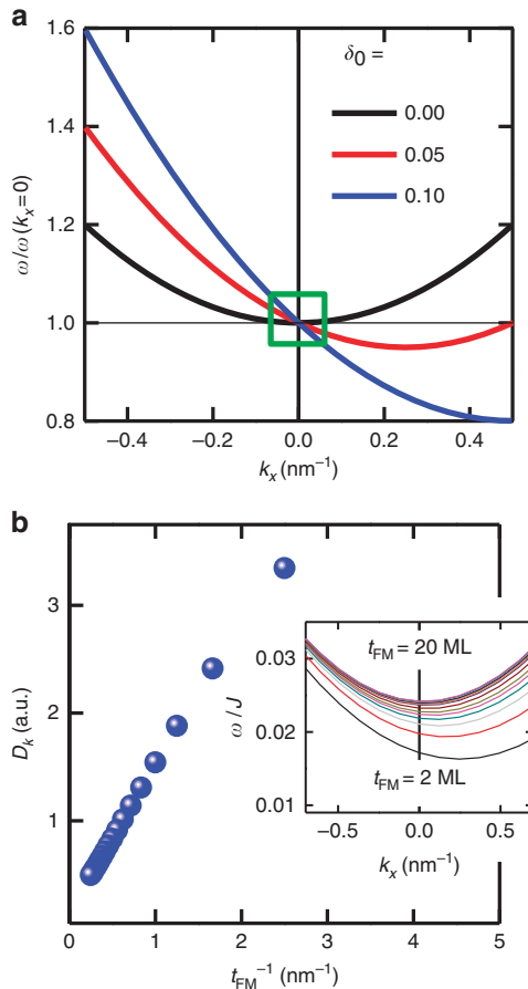
Figure 6 | Numerically calculated SW dispersion relations. (a) Calculated SW dispersion relations for different IDM energy densities. The green box indicates that SW wavevector range of our BLS experiment. (b) The IDM energy density from the SW dispersion relations as a function of t_{\text{FM}}^{-1} . Inset: calculated SW dispersion relations for various t_{\text{FM}}^{-1} from 2 ML to 20 ML when \delta_0 ( SD/J_{\text{ex}}a ) is 0.1. The vertical line indicate the k_x = 0 . The SW frequencies at k_x = 0 increase with increasing t_{\text{FM}} .
