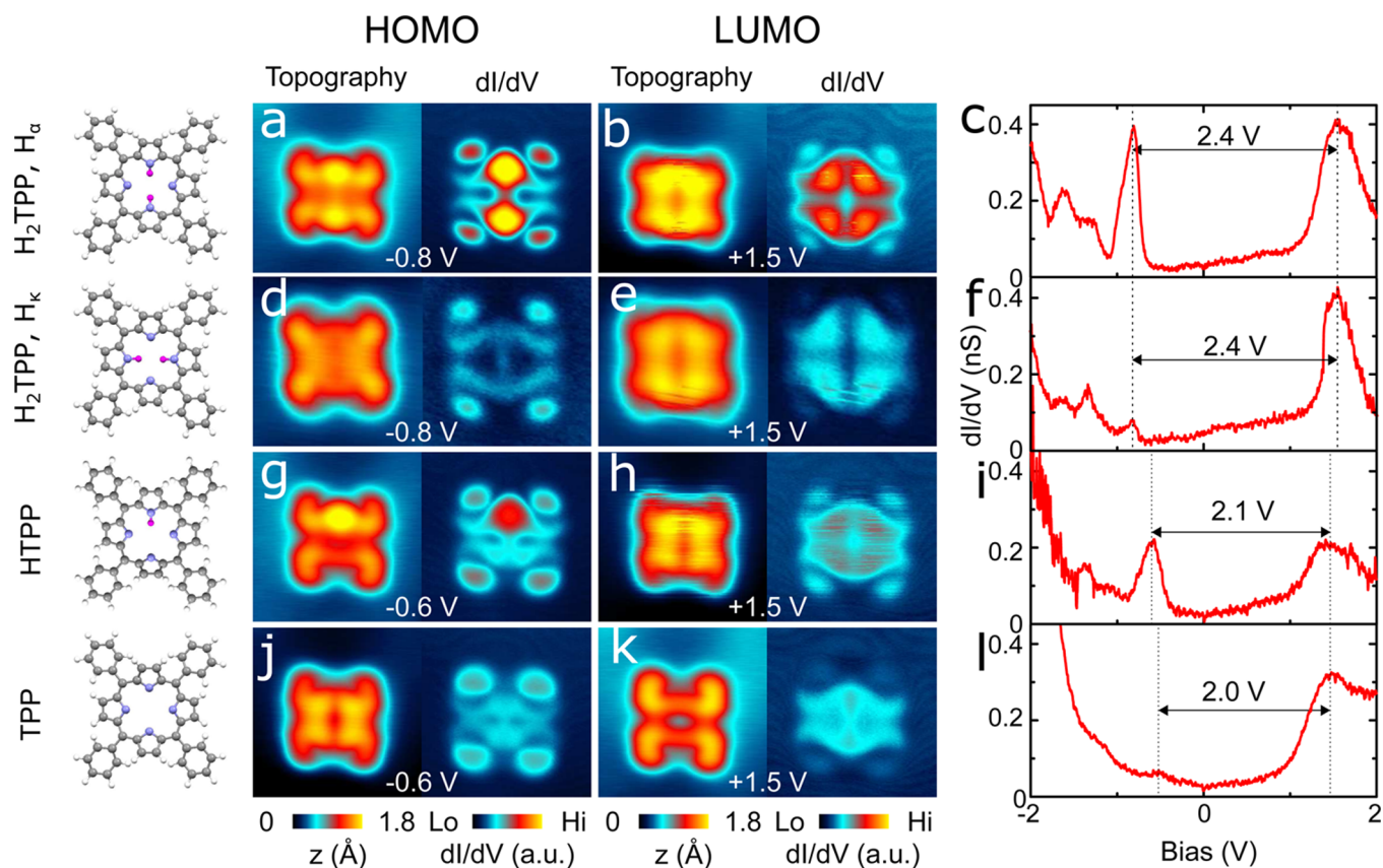
Figure 1. Topographic STM images and corresponding dI/dV maps of H_2TPP in the H_\alpha (a, b) and H_\kappa (d, e) tautomer forms and HTPP (g, h) and TPP (j, k) at different bias voltages corresponding to the HOMO and LUMO states. dI/dV spectra measured on (c) H_2TPP ( H_\alpha ), (f) H_2TPP ( H_\kappa ), (i) HTPP, and (l) TPP at a position corresponding to the bright lobe observed in the conductance map of HTPP.
