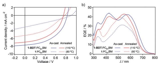
Fig. 4 (a) Current–voltage ( J – V ) characteristics of BHJ solar cells using 1:1 (w:w) blend films of 1-BDT and PC 61 BM (solid lines) and 1 and PC 61 BM (dotted lines) before (blue) and after annealing (red). (b) EQE spectra of the devices of 1-BDT :PC 61 BM (solid lines) and 1 :PC 61 BM (dotted lines) before (blue) and after annealing (red). Film thickness: 100–120 nm.
