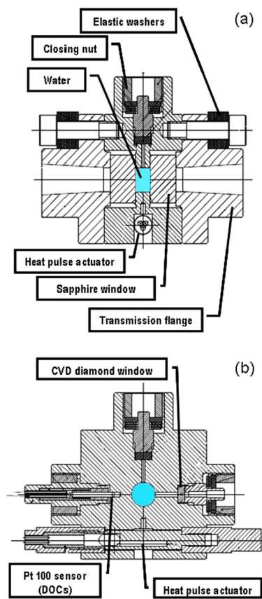
Fig. 3. (a) Side-view (with respect to Fig. 2) cross section of the HTI cell showing the optical channel for light transmission observation and details of the mechanical assembly. (b) Front-view cross section showing the optical channel for 90° light scattering measurements through the diamond window, and details of the Pt100 temperature sensor (DOCs).
