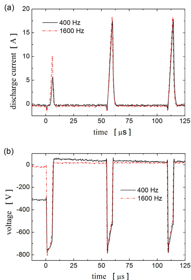
Fig. 1. Typical waveforms of the current intensity (a) and discharge voltage (b) for m-HiPIMS (sequence of three micropulses of 5 \mu\text{s} in width separated by time-off periods of 50 \mu\text{s} ) at sequence repetition frequency values of 400 and 1600 Hz, respectively.
