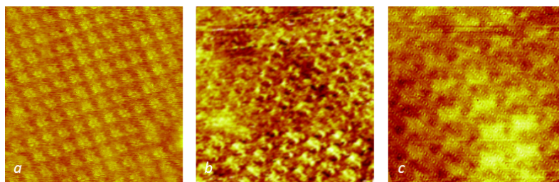
Figure 2: Structural characterization of the self-assembled PTCDI monolayers. Molecular formula of PTCDI-C13 and STM images of self-assembled monolayers on HOPG (a: 14 \times 14 nm 2 ) as-grown CVD monolayer graphene on copper foil (b: 11 \times 11 nm 2 ) and CVD graphene monolayer transferred onto a PET plate (c: 8 \times 8 nm 2 ). The typical current setpoint and sample bias were 10 pA and 800 mV, respectively. The images were acquired at the interface between the substrate and a ca. 10^{-5} M solution in phenyloctane at room temperature.
