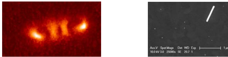
Figure 5: (Left) PEEM image obtained from a NW synthesized by CC. (Right) SEM image of the NW ( 915 nm \times 95 nm)
