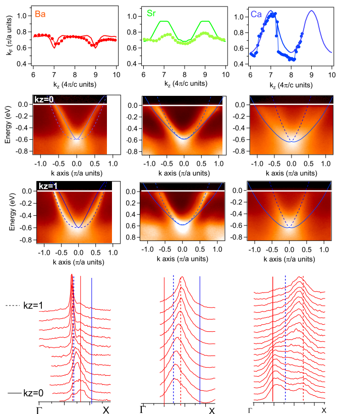
Figure 3. The different columns correspond to data measured for BaCo, SrCo and CaCo, respectively. 1st row : symbols are experimental values of k_F as a function of k_z for the d_{xz}/d_{yz} electron band. They were extracted from the maps of Fig. 2 by lorentzian fits and/or determination of local maxima. The contour expected in bulk calculation is shown as solid line. 2nd row : Energy-momentum images of dispersion along \Gamma X at k_z=0 (68eV for BaCo, 50eV for SrCo and 63eV for CaCo). k = 0 corresponds to X. Lines indicate bulk calculation at k_z=0 (solid line) and k_z=1 (dotted line) renormalized by 1.4. For CaCo, data are also shifted up by 70 meV. 3rd row : Same for k_z=1 (86eV for BaCo, 68eV for SrCo and 85eV for CaCo). 4th row : MDC stacks along \Gamma X from k_z=0 (lower spectrum) to k_z=1 (higher spectrum). Vertical lines indicate the calculated positions of k_F in bulk calculation at k_z=0 (solid) and k_z=1 (dotted) for d_{xz}/d_{yz} (red) and d_{xy} (blue).
