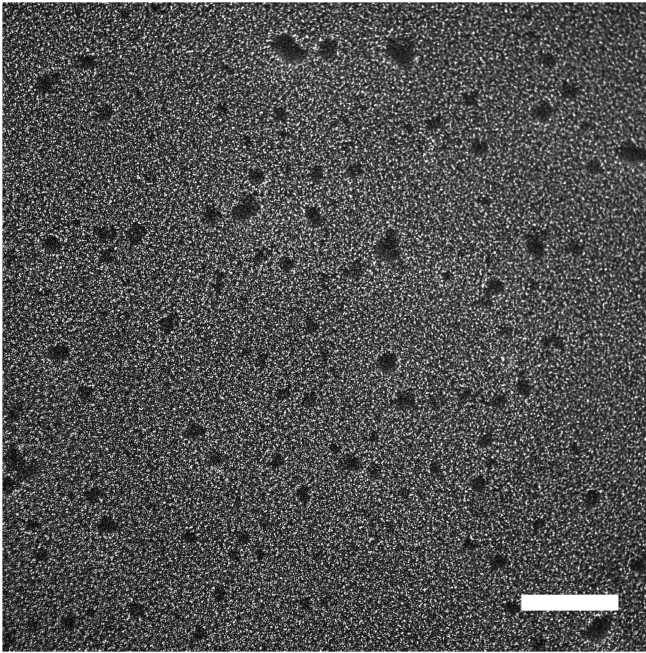
Extended Data Figure 9 | Clustering pattern during biofilm formation in swarming colonies. a , Phase-contrast image. b , Fluorescent image. Scale bars, 100 \mu\text{m} . The images were taken at about 2 cm from the inoculum after 18 h growth (Methods). The clusters (dark spots in a , or bright spots in b ) were sessile biofilms, while cells remained motile elsewhere. The colony consisted of mostly fluorescent cells. Fluorescence intensity at biofilm clusters appeared brighter than elsewhere because of
