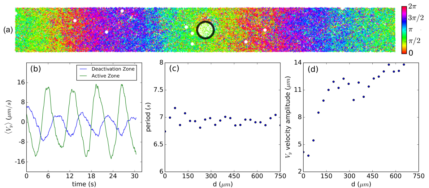
Extended Data Figure 8 | Deactivation of cell motility in mathematical model. In the simulation, we created a deactivation zone in the centre of the simulation domain (as indicated by the region inside the black circle in a ) by setting the self-propelled velocity v_0 = 0 and the entraining force f = 0 inside a circular region of area 1,000 \mu\text{m}^2 . The angular and frequency couplings k_\theta and k_\omega are also set to zero in the deactivation zone. All the parameters are the same as in Fig. 4c–e outside the deactivation zone. a , Snapshot of Supplementary Video 8 showing the deactivation zone. b , The time series of V_y components in the middle of the deactivation
