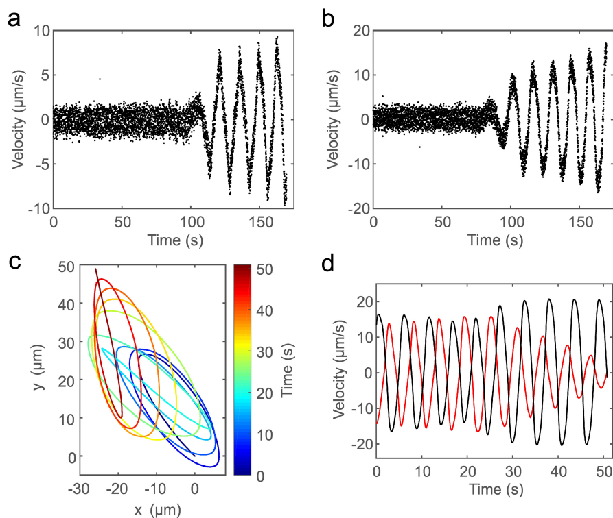
Extended Data Figure 6 | Temporal evolution of collective velocity during the emergence of collective oscillation and during chirality switching. a and b plot the x- and y-axis components of the collective velocity associated with Fig. 3b obtained by PIV analysis, respectively. Prior to the onset of collective oscillation (before about 75 s in the plots), the velocity of single cells has already recovered to normal magnitude, although the collective velocity is small. c , Chirality switching from
