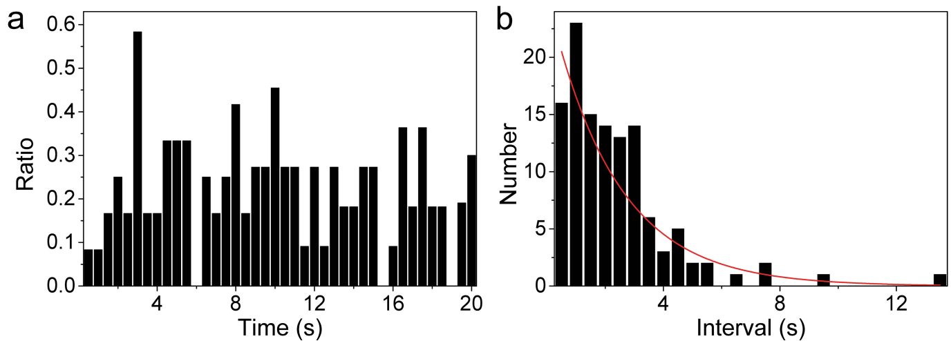
Extended Data Figure 5 | Statistics of abrupt turns made by cells undergoing collective oscillation. An abrupt turn made by a cell is defined as the change of moving direction by 135^\circ or more. During one period of collective oscillation (about 4–12 s), a cell may make several abrupt turns. a , The turning ratio, that is, the number of cells that made at least one abrupt turn during a 0.5-s interval divided by the total number of cells tracked during this 0.5-s interval, is plotted for 12 fluorescent cells undergoing collective oscillation that were tracked within a 20 s time-lapse video (see Methods for single-cell tracking). The result suggests that the
