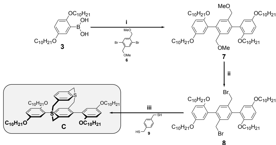
Scheme 2. Synthesis of 2,11-dithia[3.3]paracyclophane derivative C . i) Pd(PPh 3 ) 4 , K 2 CO 3 , THF/H 2 O, 95%; ii) BBr 3 , DCM, 42%; iii) 9 , KOH, DCM/MeOH, 13%
