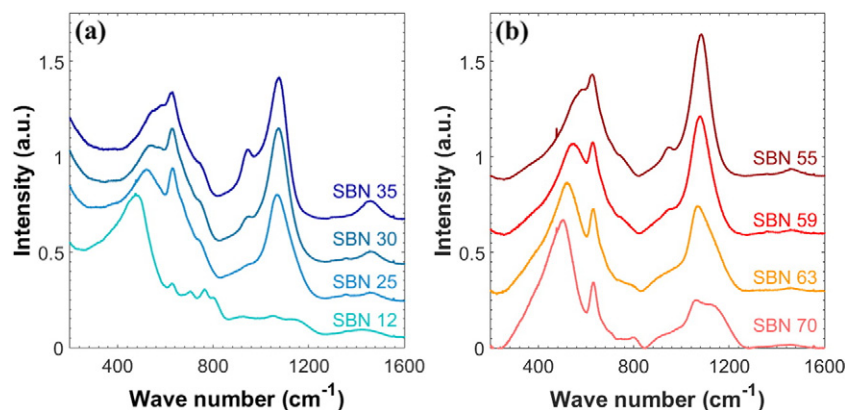
Fig. 10. The image presents Raman results concerning the K_{\text{SBN}} \sim 2.5 (a) and K_{\text{SBN}} \sim 4.5 (b) series. The curves have been offset from each other for visualization.
