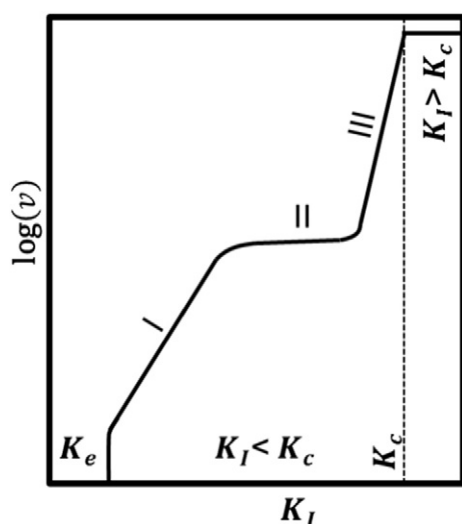
Fig. 1. Sketch of the 3 regions of sub-critical cracking commonly associated with stress corrosion cracking. In some materials, a region exists where the stresses at the crack tip are not sufficient for water to react with the crack tip, yielding an environmental limit, K_e [1].
