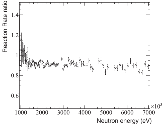
FIG. 5. The reaction rate ratio ( \frac{RR_{U8a}}{RR_{U8c}} ), plotted with 50 bins/decade.
