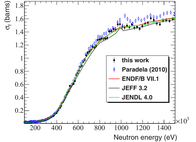
FIG. 6. The ^{237}\text{Np}(n, f) cross section, shown with 50 bins / decade, in the neutron energy range 100 keV to 1.5 MeV. The error bars correspond to the statistical uncertainties. The relative statistical uncertainty did not exceed 3% above 500 keV. The present results are compared to the latest experimental data of Paradela [3] (obtained from the same facility) and to the evaluations ENDF/B-VII.1 [23], JEFF 3.2 [25], and JENDL 4.0 [24].
