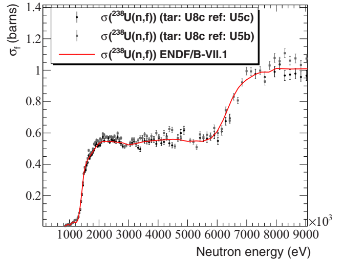
FIG. 4. The ^{238}\text{U}(n, f) cross section obtained with the small diameter targets: U8c as target and U5c (black points) and U5b as reference targets. The ENDF/B VII-1 [23] evaluation is shown for comparison. The results are given with a resolution of 50 bins / decade and the error bars correspond to the statistical uncertainties only.
