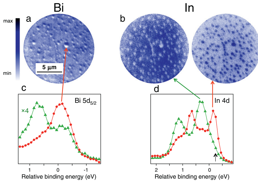
Fig. 6. 30 BL Bi/InAs(111)B sample after 10 min annealing at 300 °C: (a) Bi PEEM image averaged over the whole Bi 5d_{5/2} photoelectron spectrum; (b) In PEEM image recorded at the energy of the intensity maximum of the In 4d photoelectron spectrum, between the clusters (left) and on the clusters (right); (c) and (d) Bi 5d_{5/2} and In 4d core level spectra for two regions: between the Bi clusters (green curve with triangles) and on the Bi clusters (red curve with dots).
