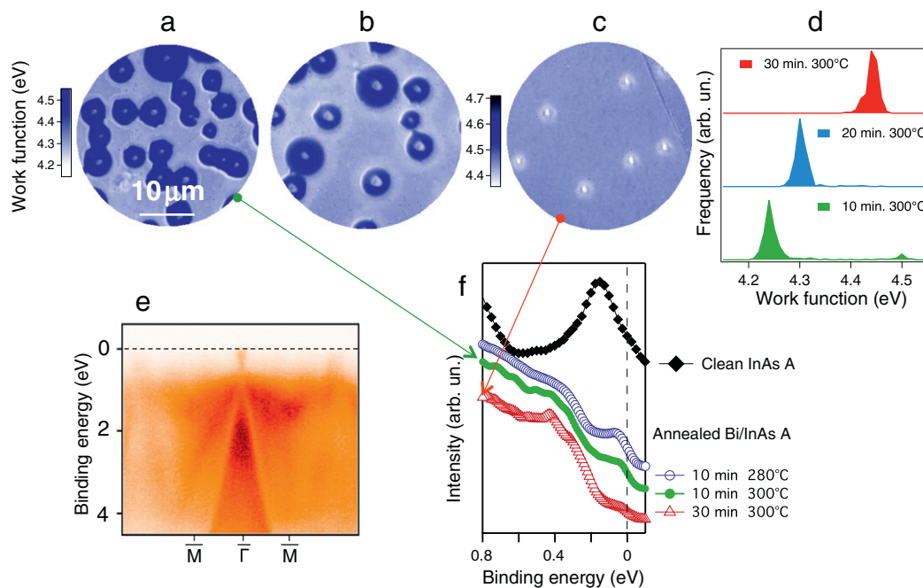
Fig. 4. 30 BL Bi/InAs(111)A sample after annealing at 300 °C: (a) work function map taken with the mercury lamp after a first 10 min annealing; (b) and (c) further annealing for 10 and 20 min, respectively; (d) work function histograms corresponding to samples (a–c); (e) ARPES spectrum in the \bar{\Gamma} - \bar{M} direction of the surface shown in (a); (f) energy distribution curve close to the Fermi level for the surfaces in (a) and (c). For comparison, the spectra corresponding to the clean InAs(111)A surface and to the 30 BL Bi/InAs(111)A surface annealed at 280 °C are also shown.
