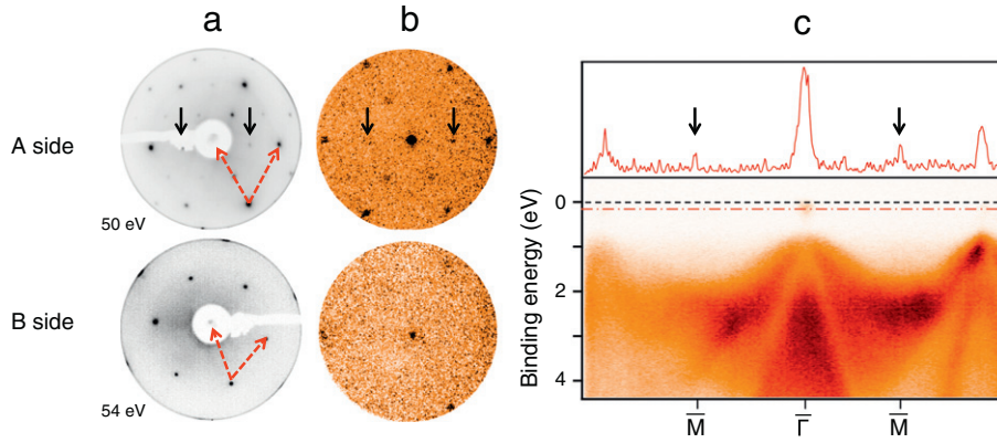
Fig. 1. Clean InAs(111): (a) LEED patterns (at 50 eV for the A side and at 54 eV for the B side). The basis vectors of the reciprocal space are shown as dashed (red) arrows; (b) k -maps near the Fermi level; (c) ARPES of the A side along the \bar{\Gamma} - \bar{M} direction (bottom panel) and intensity profile of the ARPES spectrum near (red dash-dotted line) the Fermi level (black dashed line) (top panel).
