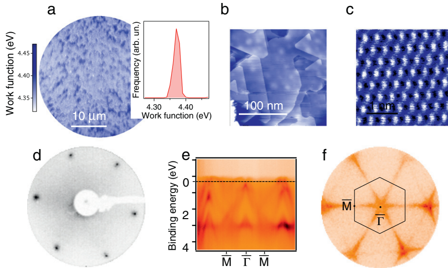
Fig. 2. 30 BL Bi/InAs(111)B: (a) work function map taken with the mercury lamp and work function histogram (inset); (b) STM image showing terraces with a six-fold symmetry; (c) STM image showing the hexagonal arrangements of the Bi atoms on a terrace; (d) Bi/InAs(111)B-(1 × 1) LEED pattern (at 33 eV); (e) ARPES in the \bar{\Gamma} - \bar{M} direction; (f) Fermi surface [the Bi(111) surface Brillouin zone with relevant high symmetry points is shown for reference].
