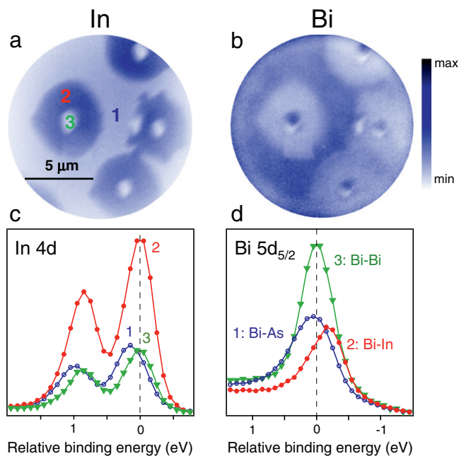
Fig. 5. 30 BL Bi/InAs(111)A sample after a 10 min annealing at 300 °C: (a) In 4d and (b) Bi 5d PEEM images; (c) In 4d and (d) Bi 5d_{5/2} photoelectron spectra corresponding to the regions 1, 2 and 3 of (a).
