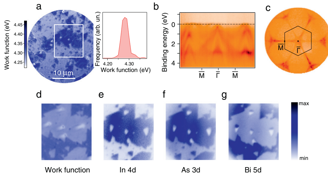
Fig. 3. 30 BL Bi/InAs(111)A sample after annealing at 230 °C: (a) work function map taken with the mercury lamp and work function histogram; (b) ARPES in the \bar{\Gamma} - \bar{M} direction; (c) Fermi surface [the Bi(111) surface Brillouin zone with relevant high symmetry points is shown for reference]; (d) work function image for the region indicated by the white frame in (a); (e–g) In 4d, As 3d and Bi 5d PEEM corresponding energy filtered images of the white frame area.
