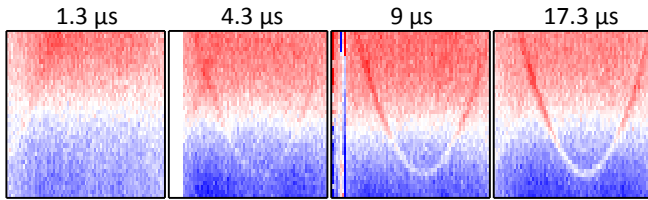
Figure 9: Spectroscopy Andreev transition of the second channel ( 2eV_J = 2E_{A2} ) near \varphi = \pi , with increasing delay \Delta t between prepulse and measurement pulse (1.3 to 17.3 \mu\text{s} ). In each sub-spectrum, the x-axis spans the interval 0.7\pi < \varphi < 1.3\pi , the y-axis 1.58\Delta < 2eV_J < 1.66\Delta (red box in Fig. 8(a)).
