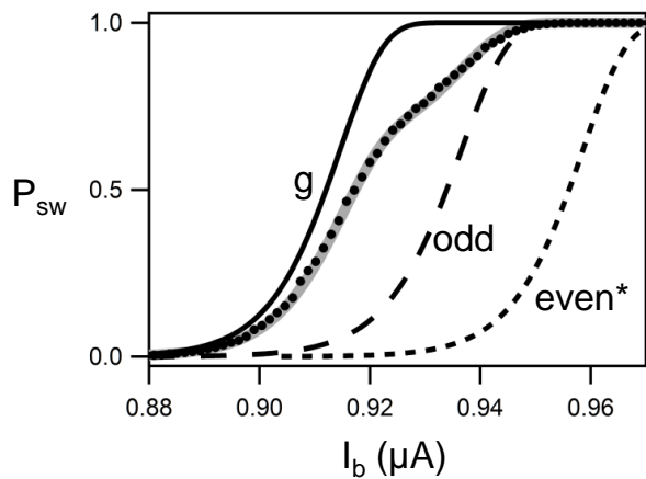
Figure 4: Dots: Switching probability P_{sw}(I_b) measured near the minimum of the Andreev transition line at 2E_{A1} ( 2eV_J = 0.24\Delta , \varphi = 1.02\pi ). Solid line: calculated P_{sw}(I_b) with the two channels in the ground state (corresponding to a total current in the SQUID junction I_b - I_{A1} - I_{A2} ). Dashed line: calculated P_{sw}(I_b) with the first channel in an odd state (corresponding to a total current in the SQUID junction I_b - I_{A2} ). Grey curve: fit of the data with sum of the two previous curves with weights 0.63 and 0.37. Short-dashed line: calculated P_{sw}(I_b) with the first channel in the even excited state (corresponding to a total current in the SQUID junction I_b + I_{A1} - I_{A2} ). A finite probability to find the channel in the even excited state would have resulted in a contribution of the short-dashed line to the data.
