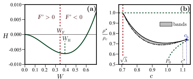
FIG. 2. (a) Sketch of the motion of an oscillating point particle in the effective potential H(W) for P_0 = 1 , \rho_c = 1 , \lambda = 0.5 , \xi = 1 , c = 0.9 and \rho^* = 0.7 . The system loses or gains energy H when F'(W) > 0 or F'(W) < 0 . (b) Band phase diagram for the same parameters. Non-linear bands exist only in the grey region. The dashed lines correspond to the conditions W_H > 0 , and W_F > 0 . For c < c^* , the black full line corresponds to the supercritical Hopf-bifurcation. Polar-liquid droplets states are observed only at c = c_h .
