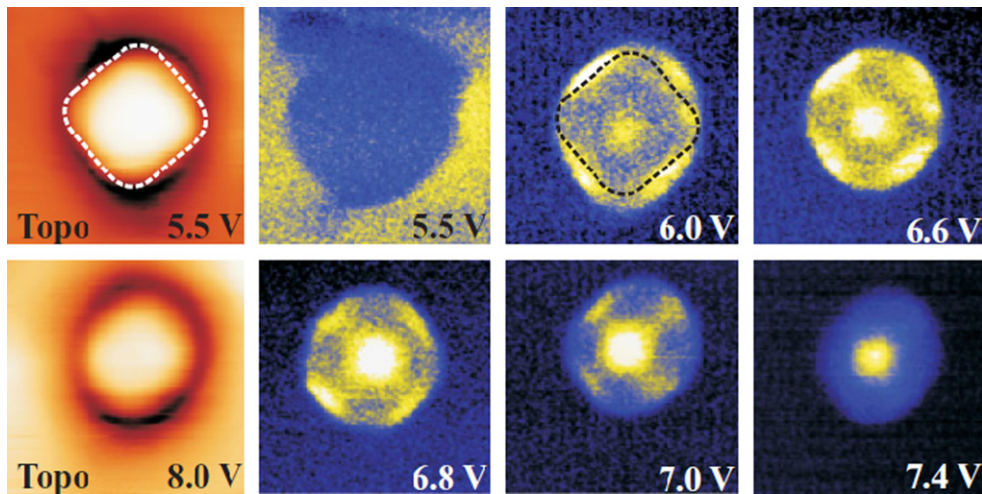
Fig. 4. STM topographic images and photon maps of an Ag particle on MgO/Mo(001) taken as a function of sample bias ( I_T = 1 nA, 8\text{ nm} \times 8\text{ nm} ). The variations of luminescence distribution reflect the different in-plane and out-of-plane excited plasmon modes. Adapted from Myrath et al. [73].
