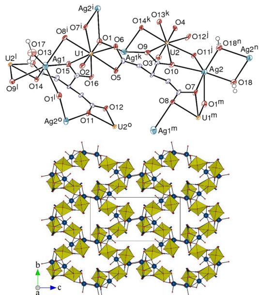
Figure 2. Top: View of compound 2 . Displacement ellipsoids are drawn at the 50% probability level. The solvent molecule and carbon-bound hydrogen atoms are omitted. Symmetry codes: i = x - 1, y, z ; j = 1 - x, y + 1/2, 1/2 - z ; k = -x, y + 1/2, 1/2 - z ; l = -x, y - 1/2, 1/2 - z ; m = x + 1, y, z ; n = 2 - x, 1 - y, 1 - z ; o = 1 - x, y - 1/2, 1/2 - z . Bottom: View of the 3D framework with the uranium coordination polyhedra colored yellow and silver atoms shown as blue spheres; the 2D honeycomb subunits are viewed edge-on; solvent molecules and hydrogen atoms are omitted.
