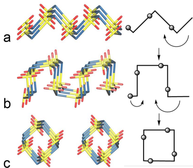
Figure 3. Nodal representation of the triangular-grooved network in 1/4 (a), the square-grooved network in 2 (b), and the tubular chains in 3 (c), and schematic representation of the transformation. Yellow: uranium, red: oxygen, blue: tricarballylate ligand.
