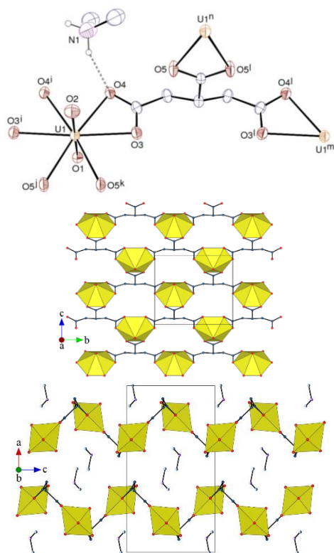
Figure 1. Top: View of compound 1 . Displacement ellipsoids are drawn at the 30% probability level. The solvent molecule and carbon-bound hydrogen atoms are omitted, and only one position of the disordered counterion is shown. The hydrogen bond is shown as a dashed line. Symmetry codes: i = x, 3/2 - y, z ; j = 1/2 - x, y + 1/2, z - 1/2 ; k = 1/2 - x, 1 - y, z - 1/2 ; l = x, 1/2 - y, z ; m = x, y - 1, z ; n = 1/2 - x, 1 - y, z + 1/2 . Middle: View of the 2D assembly. Bottom: View of the packing. Uranium coordination polyhedra are colored yellow and solvent molecules and hydrogen atoms are omitted in the last two views.
