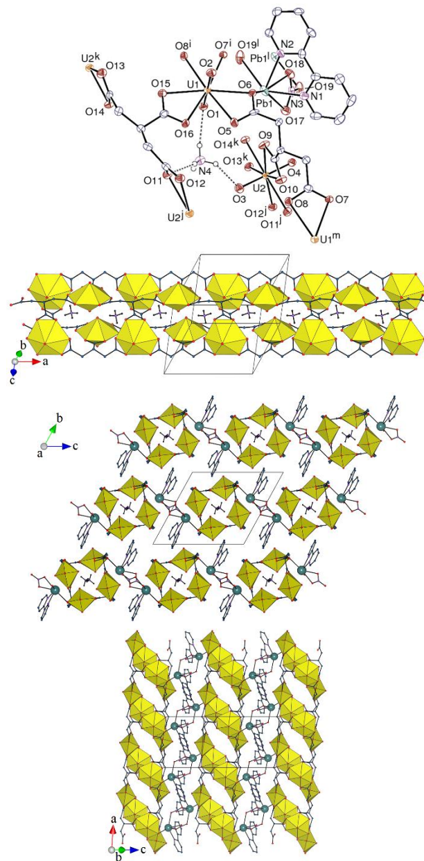
Figure 4. Top: View of compound 3 . Displacement ellipsoids are drawn at the 40% probability level. Carbon-bound hydrogen atoms are omitted and hydrogen bonds are shown as dashed lines. Symmetry codes: i = x + 1, y, z ; j = 1 - x, 1 - y, 1 - z ; k = 2 - x, 1 - y, 1 - z ; l = 2 - x, 1 - y, 2 - z ; m = x - 1, y, z . Middle: View of one tubular subunit. Bottom: Two views of the packing parallel and perpendicular to the tubules axis, with the uranium coordination polyhedra colored yellow, lead atoms shown as green spheres, and hydrogen atoms omitted, except for those of the NH_4^+ counterions.
