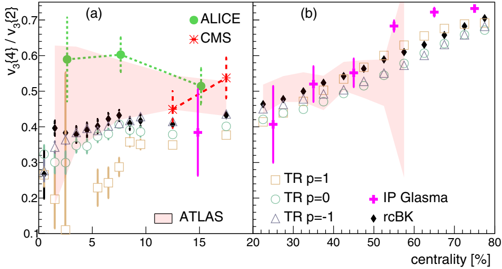
FIG. 3. Test of initial condition models using v_3\{4\}/v_3\{2\} measured in 2.76 TeV Pb + Pb collisions: (a) up to 20% centrality; (b) between 20% and 80% centrality. Stars: CMS data [47]. Full circles: ALICE data [41]. Shaded band: ATLAS data [24]. ALICE and CMS data are not shown in panel (b) for the sake of readability, but are compatible with ATLAS data. Remaining symbols correspond to values of \varepsilon_3\{4\}/\varepsilon_3\{2\} from several models of initial conditions. Open symbols: T R ENTo, with p = -1 (triangles), p = 0 (circles), p = 1 (squares). Full crosses: IP-Glasma [18]. Full diamonds: Monte Carlo rcBK [16].
