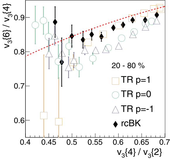
FIG. 4. Predictions for v_3\{6\}/v_3\{4\} in 2.76 TeV Pb + Pb collisions, from several models of initial conditions, in the 20–80% centrality range. Empty symbols: Predictions of Tr Trento with p = 1 (squares), p = 0 (circles), and p = -1 (triangles). Full diamonds: Prediction of Monte Carlo rcBK [16]. The red dashed line is the prediction of the power distribution [50].
