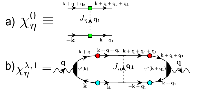
FIG. 5. (color online) a) \chi_S^0 is the single segment of the ladder diagrams describing the \eta -mode. This term is evaluated in the formula (12) in the section II C 1. b) \chi_\eta^{\lambda,1} is the first term of the series of ladder diagram. \gamma_k^\lambda is the Raman vertex in the \lambda symmetry. This term is evaluated in the formula (14) in the section II C 2. Both terms are evaluated in the approximation of a momentum and frequency independent J_\eta .
