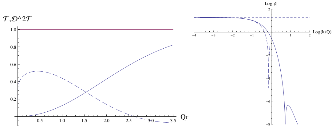
Fig. 1. Positivity and unitarity tests of the McLerran-Venugopalan model with running coupling.
