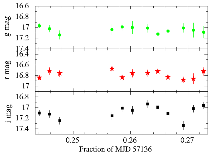
Fig. 3. From top to bottom, gri light curves obtained with the REM telescope on Apr. 24, 2015. Errors are indicated at the 68% confidence level.
