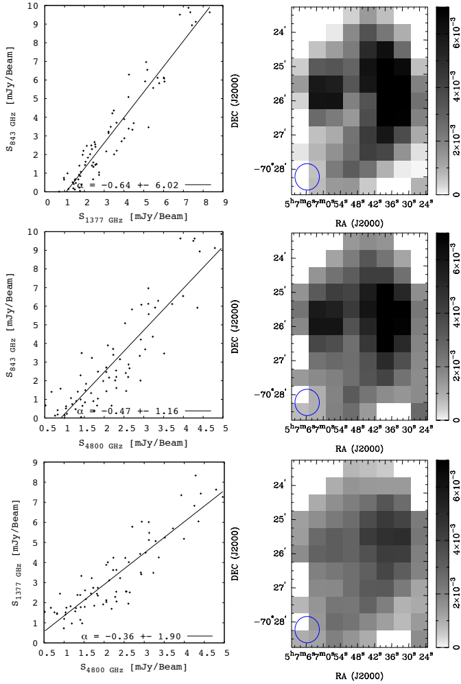
Fig. 6. Left: T-T plots of MCSNR J0506–7025 between 36–20 cm, 36–6 cm, and 20–6 cm ( top to bottom ). Right: intensity images showing the region and strength of the emission from 36, 20, and 6 cm images ( top-to-bottom ).
