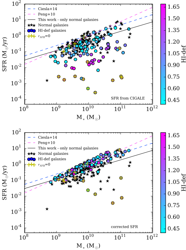
Fig. 9. Relation between the SFR and M_* of the HRS subsamples. Black stars are the normal galaxies, filled circles are the HI-deficient galaxies color-coded according to the \text{HI-def} parameter. Yellow crosses point out the sources for which r_{\text{SFR}} = 0 . Main sequence relations found at z = 0 are shown in dashed lines: in blue the one from Ciesla et al. (2014), in red the relation of Peng et al. (2010), and the relation derived in this work is the black solid line. Top panel: observed relation obtained with CIGALE. Bottom panel: estimated positions of the HI-deficient galaxies before interaction with the environment obtained after correcting their instantaneous SFR with the r_{\text{SFR}} parameter.
