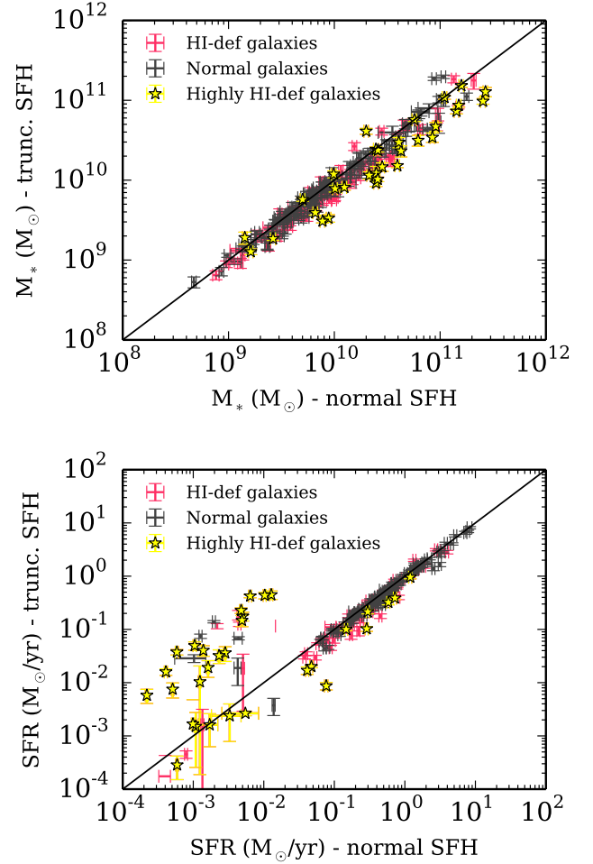
Fig. 6. Comparison between the stellar masses (top panel) and SFR (bottom panel) obtained using the truncated and normally delayed SFH. Normal galaxies are shown in gray, whereas HI-deficient and highly deficient galaxies (with HI-def ≥ 1) are shown in red and yellow, respectively. The black solid lines represent the one-to-one relationship.
