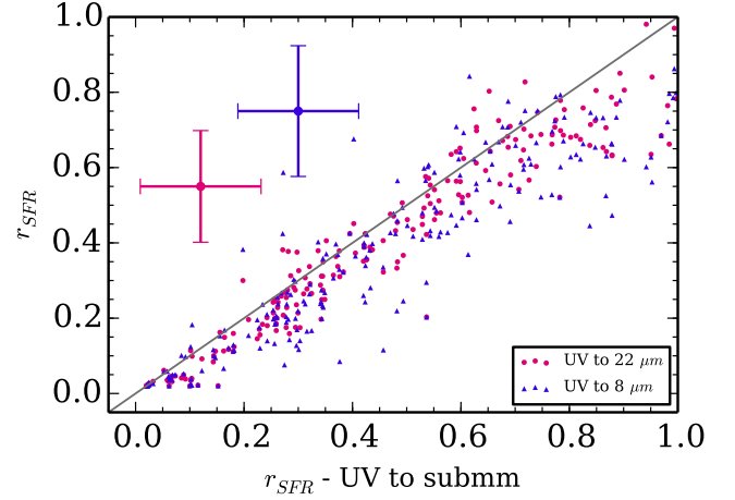
Fig. 11. Impact of the photometric coverage on the derivation of the r_{\text{SFR}} parameter. Pink points show the relation between the values obtained when the photometric coverage stops at 22 \mu\text{m} and the values obtained from a full coverage. The purple points show the relation when the photometric coverage stops at 8 \mu\text{m} . Mean error bars are shown for both subsets.
