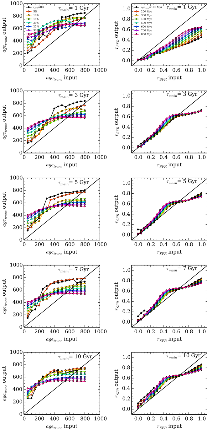
Fig. 12. Results of the z = 2 mock catalog analysis for the two parameters age_{\text{trunc}} and r_{\text{SFR}} . The five left panels present the constraint on age_{\text{trunc}} for five different \tau_{\text{main}} (1, 3, 5, 7, and 10 Gyr). The colored lines corresponds to different values of r_{\text{SFR}} . The five righthand panels display the constraint on r_{\text{SFR}} for the same five values of \tau_{\text{main}} (1, 3, 5, 7, and 10 Gyr), the colored lines corresponding to different age_{\text{trunc}} . On each panel, the black solid line is the one-to-one relationship.
