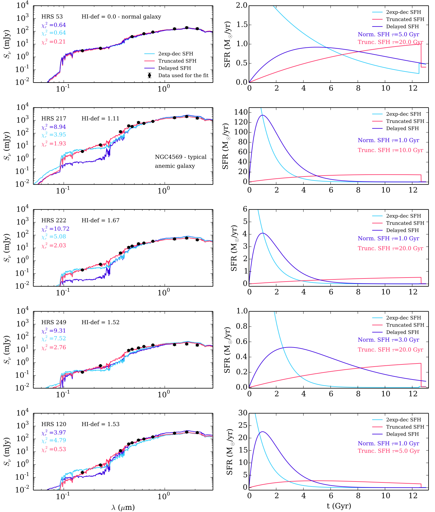
Fig. 2. Left column: examples of best fits obtained with CIGALE for one normal and four HI-deficient HRS galaxies using three different SFH assumptions: a delayed SFH (navy blue), a 2-exponentially decreasing SFH (cyan), and a truncated delayed SFH (red). Right column: for each galaxy, the output best fit SFH obtained for the three different assumptions made.
