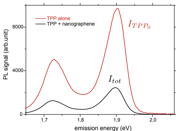
a) Quenching effect of graphene on TPP PL signal for a concentration of 8 \mu\text{mol.L}^{-1}
