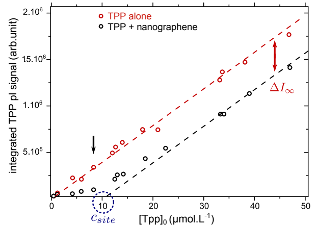
b) PL signal vs concentration with and without graphene sheets (the black arrow highlights the 8 \mu\text{mol.L}^{-1} samples)
