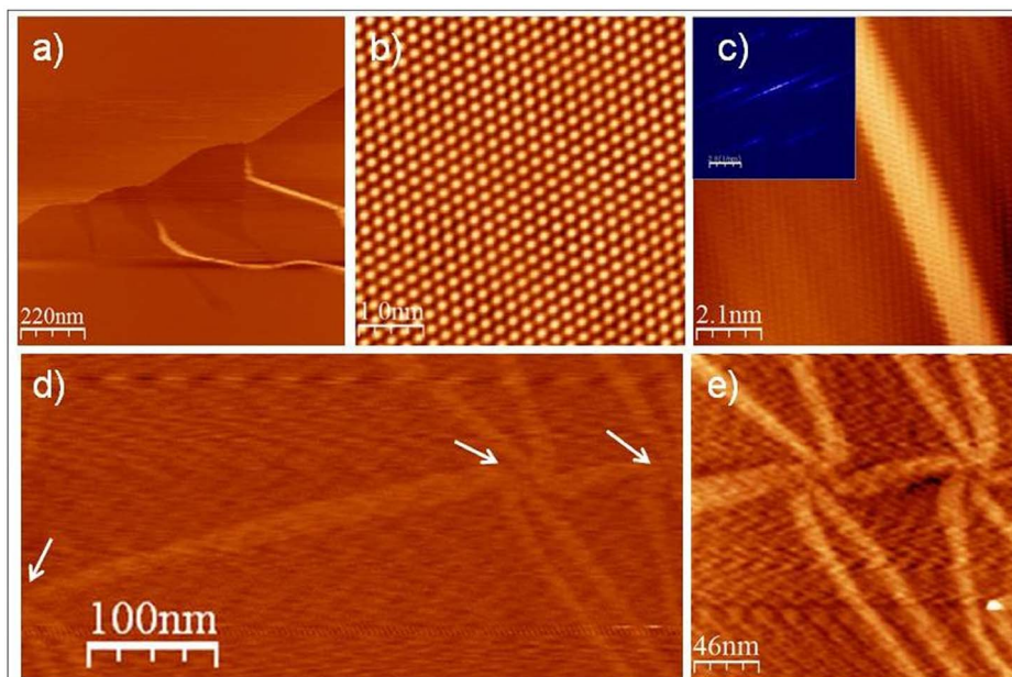
Figure 2 | Morphology of trilayer graphene. (a) Large STM image ( -1.7 V, 1 nA) of trilayer graphene (b) Triangular type structures ( 5 \times 5 nm 2 ), (c) An STM image of corrugated graphene with nearly periodic ripples of nanometer wavelength (inset Fourier transform of the STM image) (d) STM image of three interconnected flower-shaped structures, (e) STM image of two interconnected flower-shaped domains. V_s = 0.05 V, I_t = 200 pA) for (b - e).
