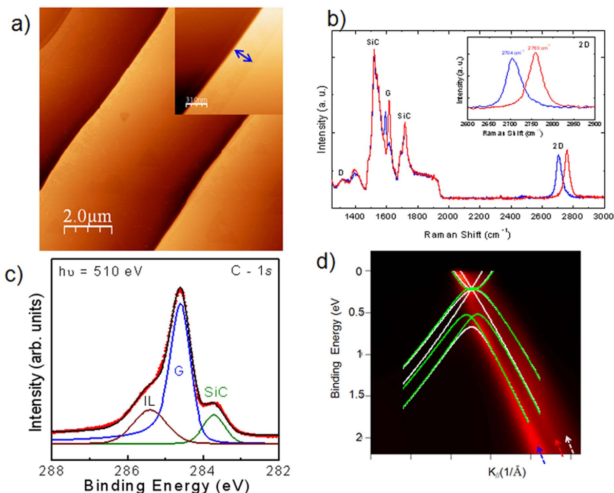
Figure 1 | Structural and Electronic Properties of Epitaxial trilayer graphene. (a) Typical AFM image of trilayer graphene, (b) Raman spectra of the graphene sample (blue line) and of step edge (red line). Contributions at the G and 2D bands are observed, together with a very low signal at the defect band D, (c) C\ 1s XPS spectra for epitaxial graphene annealed at 1550^\circ\text{C} at h\nu = 510\ \text{eV} . XPS measurements were performed at \phi = 45^\circ emergency angle with respect to the sample normal, (d) ARPES spectra along the \Gamma K direction of the graphene trilayer, together with theoretical calculation of ABA and ABC stacking (white and green, respectively). From the shift of the Dirac Energy we extract E_D = 0.2\ \text{meV} , measured with respect to the Fermi energy.
