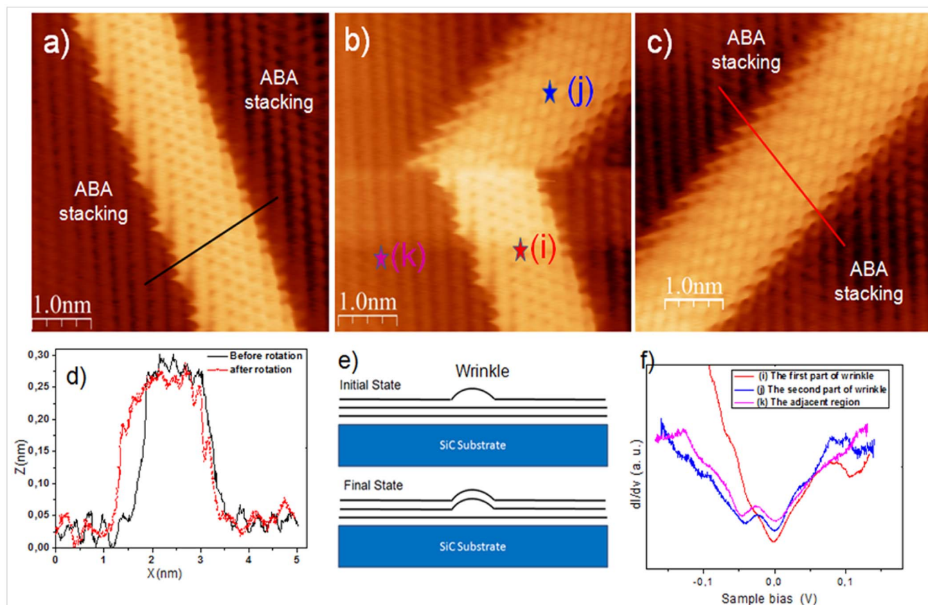
Figure 4 | Different configurations of the wrinkles. (a) STM image taken on an isolated wrinkle ( V_s = -0.05 V, I_t = 0.2 nA): honeycomb structure on the wrinkle and triangular pattern on the adjoining graphene region; (b) STM image ( V_s = -0.05 V, I_t = 0.2 nA) showing the partial rotation of the wrinkle under a tip-surface interaction effect (c) STM image ( V_s = -0.05 V, I_t = 0.2 nA) showing that the wrinkle has entirely rotated by 60^\circ from its original orientation; (d) Height profiles corresponding to the black (before rotation of the wrinkles) and red (after rotation of the wrinkles) lines in (a and c); (e) Schematic showing the modification of the wrinkle after the rotation; (f) Spatially averaged dI/dV curves at three different regions in figure 4(b).
