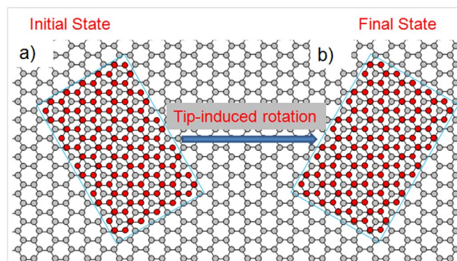
Figure 5 | Structure of the wrinkles on the graphene layer. Schematic representation of the proposed diffusion mechanism through rotation of the wrinkle from the initial to the final states: (a) initial state (b) final state of the wrinkle.
