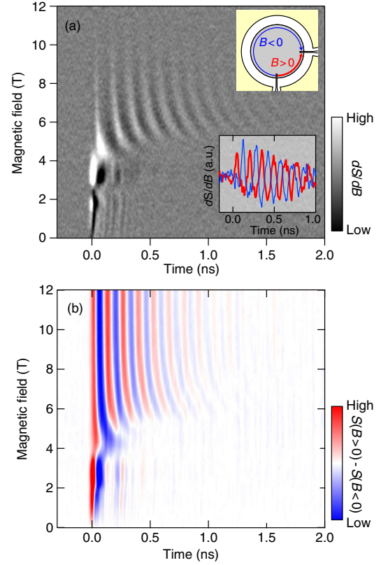
FIG. 3 (color online). Results of time domain measurement. (a) Differential signal ( dS/dB ) of the 200- \mu\text{m} sample as a function of time and B . Inset shows dS/dB at B = 6.5 T (red thick trace) and B = -6.5 T (blue trace). The chirality of the EMP orbital motion is counterclockwise (clockwise) for positive (negative) B . (b) S(B > 0) - S(B < 0) for the 200- \mu\text{m} sample.
