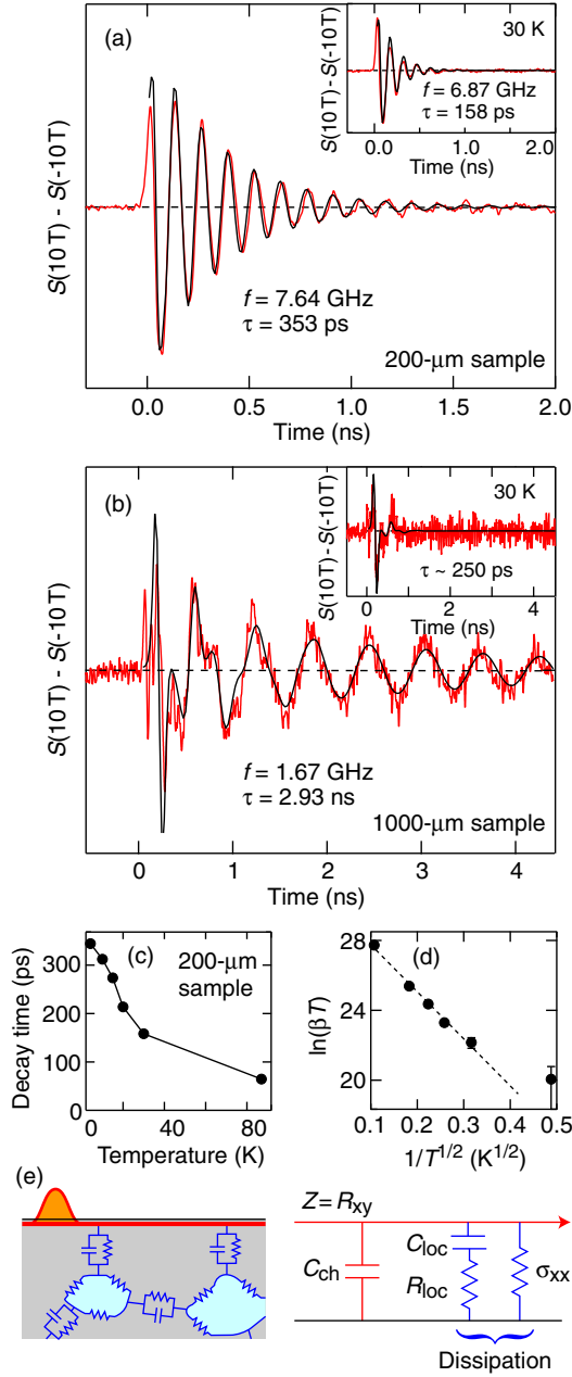
FIG. 4 (color online). Temperature dependence of EMP decay. (a) and (b) S(10\text{ T}) - S(-10\text{ T}) at T = 4\text{ K} for the 200- and 1000-μm samples, respectively. Insets show the traces at T = 30\text{ K} . Black traces represent results of the simulation (details are indicated in the main text). (c) \tau for the 200-μm sample as a function of T . (d) \ln(\beta T) as a function of T^{-1/2} . Linear fit gives T_0^{1/2} = 26.9 \pm 1.4\text{ K}^{1/2} in Eq. (3). (e) Illustration and equivalent circuit model for the EMP dissipation through interaction with localized states in the interior of graphene.
