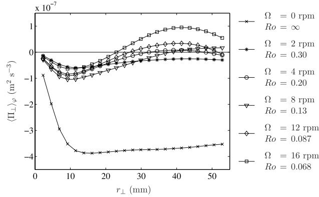
FIG. 5. Azimuthal average of the horizontal energy flux, \langle \Pi_{\perp} \rangle_{\phi} , as a function of horizontal separation r_{\perp} and for various rotation rates \Omega . These data are computed from measurements in the horizontal plane. A negative value (respectively, positive) corresponds to a direct (respectively, inverse) energy transfer.
