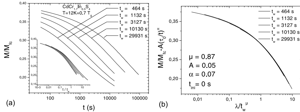
Figure 1. (a) Thermoremanent magnetization relaxations at 0.7T_g on the thiospinel CdCr_{1.7}In_{0.3}S_4 spin glass ( T_g = 16.7 K); (b) scaling of the previous relaxation curves (see text for details).
