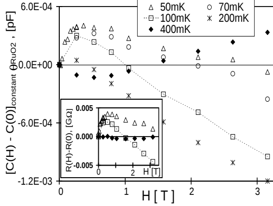
FIG. 2: \delta C(H) measured by keeping \theta_{\text{RuO}_2} constant while increasing H (the various T labeling the curves are at H = 0 ). Inset : Corresponding data for \delta R(H) (same symbols). The fact that \delta R(H) and \delta C(H) do not vanish at the same H cannot be explained by using only \delta T(H) effects but implies that a \delta \epsilon_r(H) dependence exists in the sample. The error bars c_{\text{noise}} = \pm 10^{-5} pF and r_{\text{noise}} = \pm 10^{-5} G \Omega are much smaller than the data symbols.
