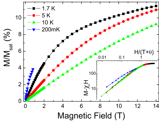
FIG. 3. (Color online) Normalized magnetization ( M_{sat} = 5583 emu) measured versus field in a VSM for three characteristic temperatures. The magnetization data at 0.2 K are also reported from the inset of Fig. 2. In the inset, for the same temperatures, M - \chi_i H versus H/(T + \theta) with \chi_i = 1.25 \times 10^{-3} cm 3 /mol Cu and \theta = 1.3 K.
