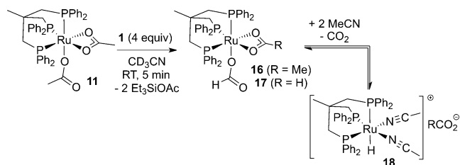
Scheme 3. Reaction of the complex 11 with 1 in acetonitrile.
