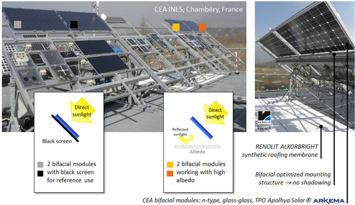
Fig. 7. Description of the CEA-INES outdoor bifacial setup
