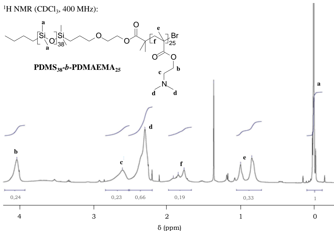
Figure 2. ^1\text{H} NMR spectra of \text{PDMS}_{38}\text{-}b\text{-PDMAEMA}_{25} in \text{CDCl}_3
