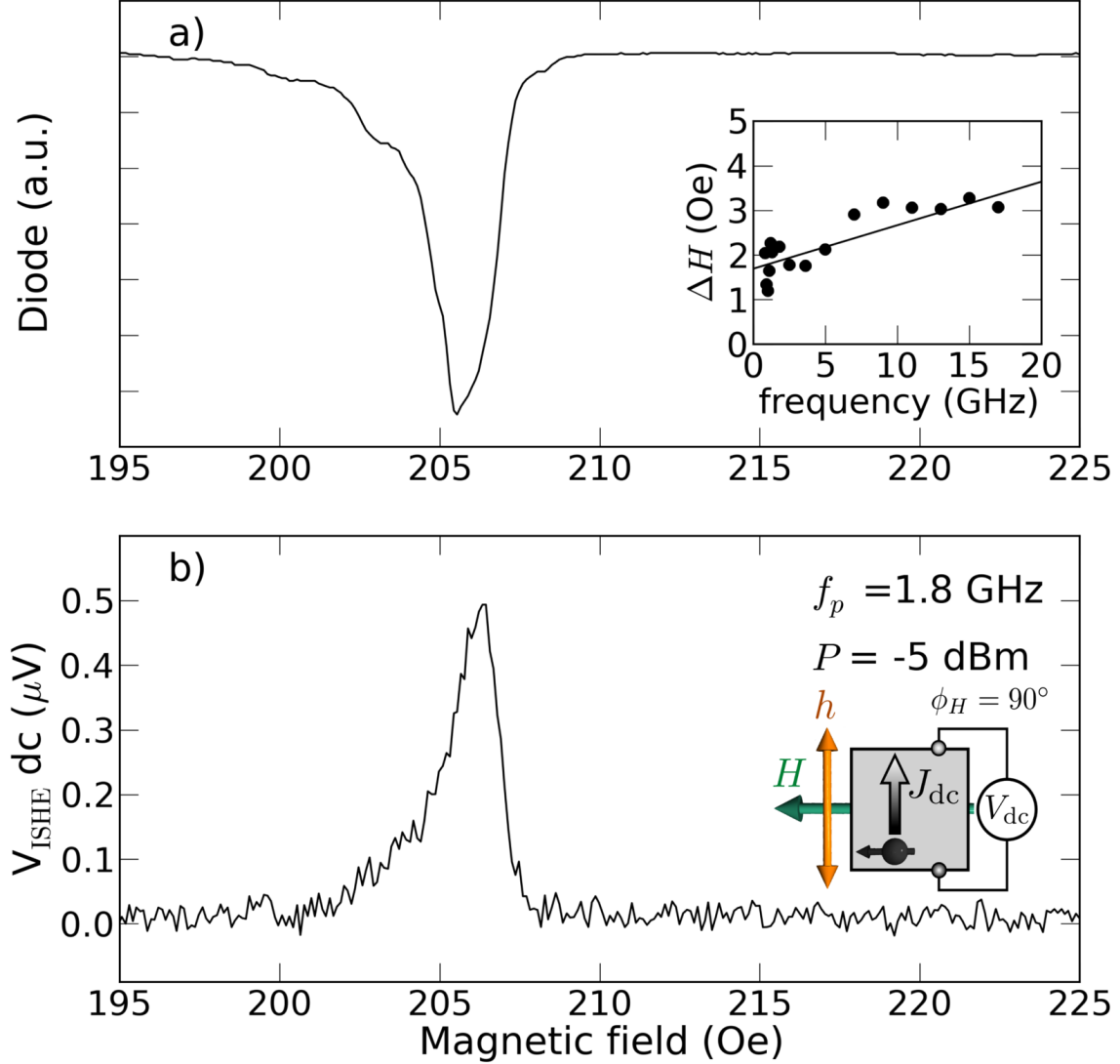
FIG. 2. (Color online) Standard FMR detected using dc ISHE voltage. The pumping field h oscillating at f_p = 1.8 \text{ GHz} is oriented perpendicularly to the static magnetic field H . (a) Larmor absorption peak of the uniform mode detected with a diode (the inset shows the dependence of the linewidth on frequency). (b) Corresponding dc ISHE voltage measured perpendicularly to H (the inset shows the geometry of the experiment).
