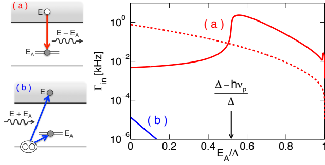
FIG. 3: Left: Schematic representation of processes adding a quasiparticle in the Andreev level. Right: the emission processes (a) rates, denoted by \Gamma_{\text{in}}^{(a)} in the text, are given by the red curves for photons (full line) and phonons (dashed lines). The processes (b) involving the breaking of a Cooper pair (blue line in the plot) are much less efficient. The one involving the phonons is below this scale. Same parameters as in Fig. 2.
