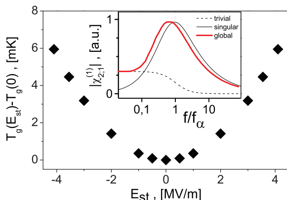
FIG. 3. (Color online) Inset: Qualitative picture of the trival, singular, and global \chi_{2,1}^{(1)} . Main panel: Evolution of T_g with E_{st} by the quantity 3\kappa E_{st}^2 . The size of the points is larger than the \pm 2.5\% uncertainty on \kappa .
